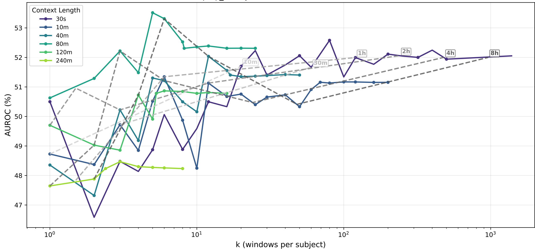
psqi_binary · lstm — AUROC (%) vs k
