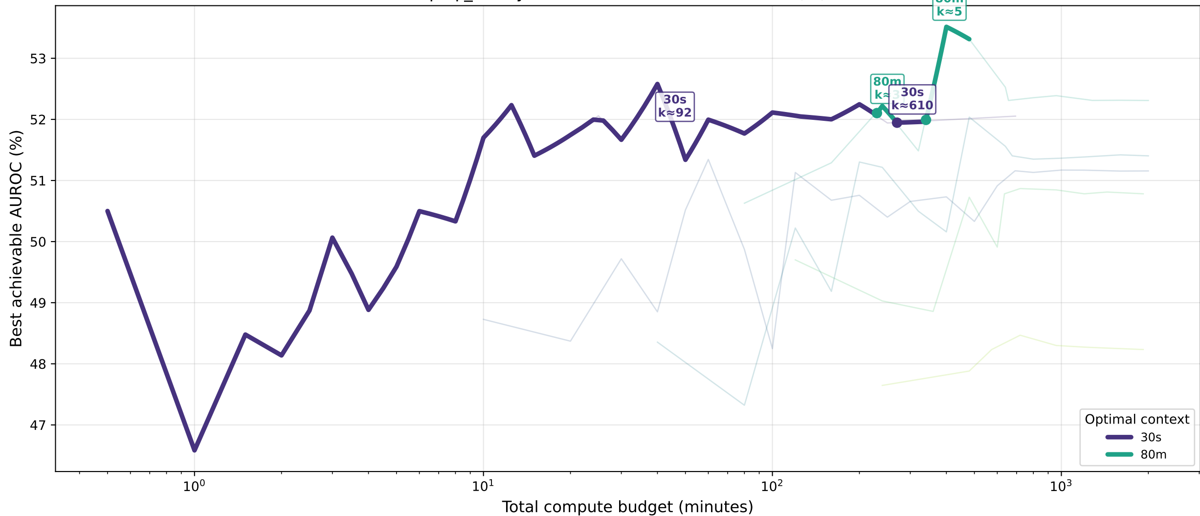
psqi_binary · lstm — Pareto Front: AUROC (%)
