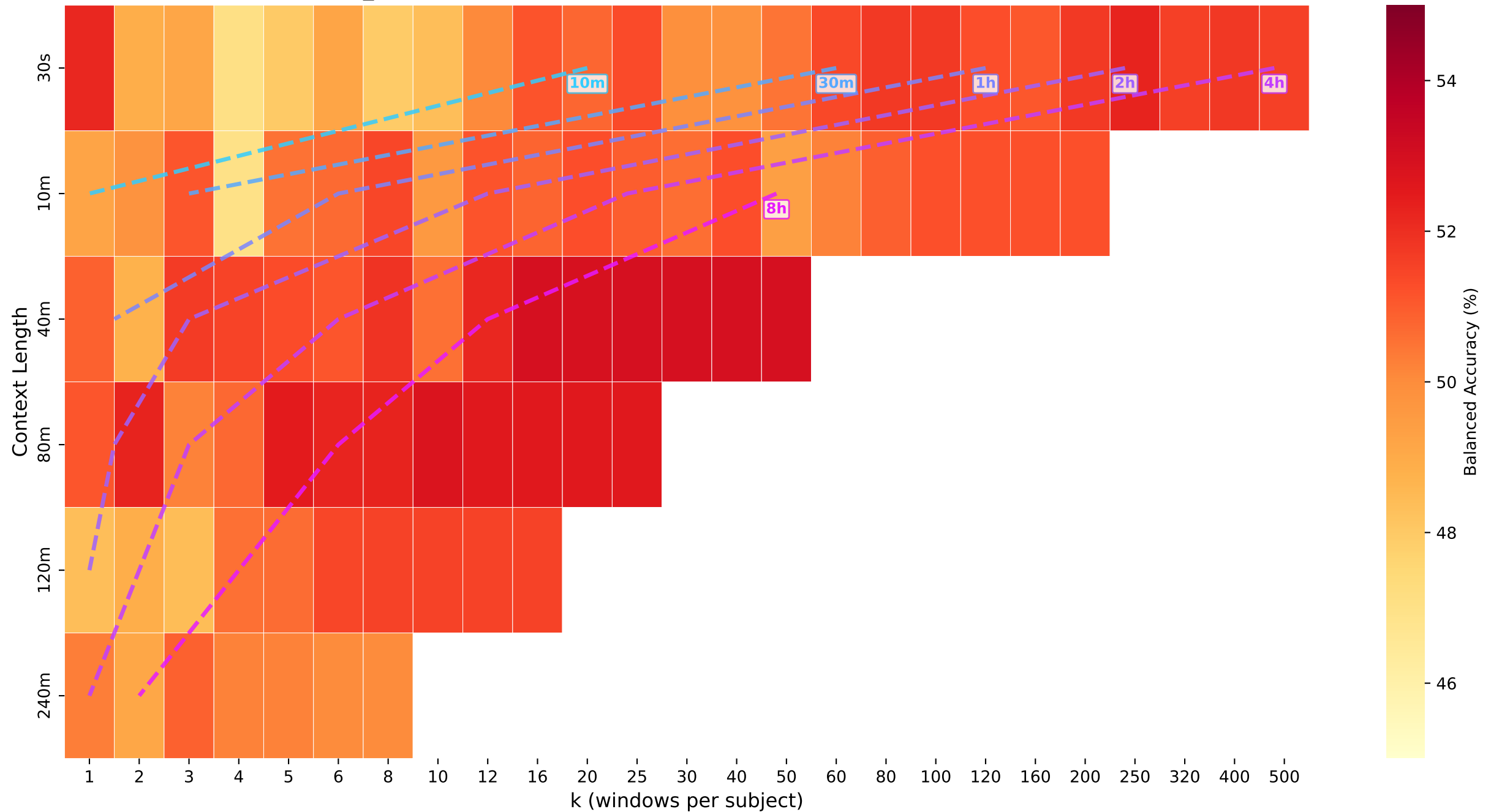
psqi_binary · lstm — Iso-Compute Heatmap: Balanced Accuracy (%)
