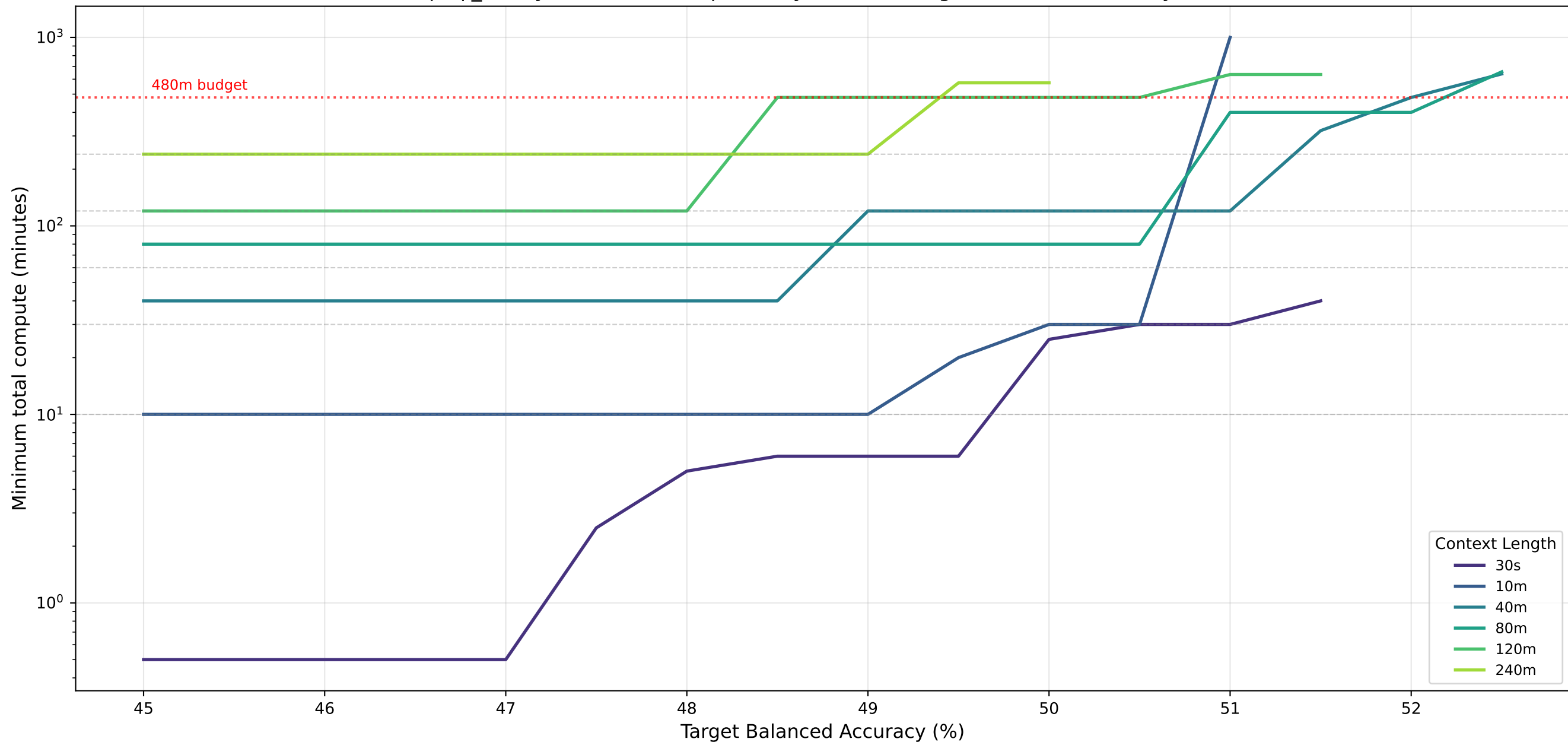
psqi_binary · lstm — Cheapest Way to Reach Target Balanced Accuracy (%)
