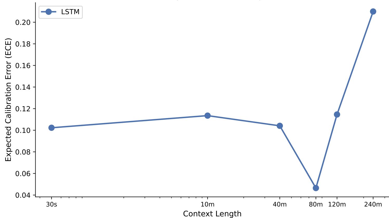
ECE vs Context Length — psqi_binary (K=10) Lower is better; longer context should improve calibration
