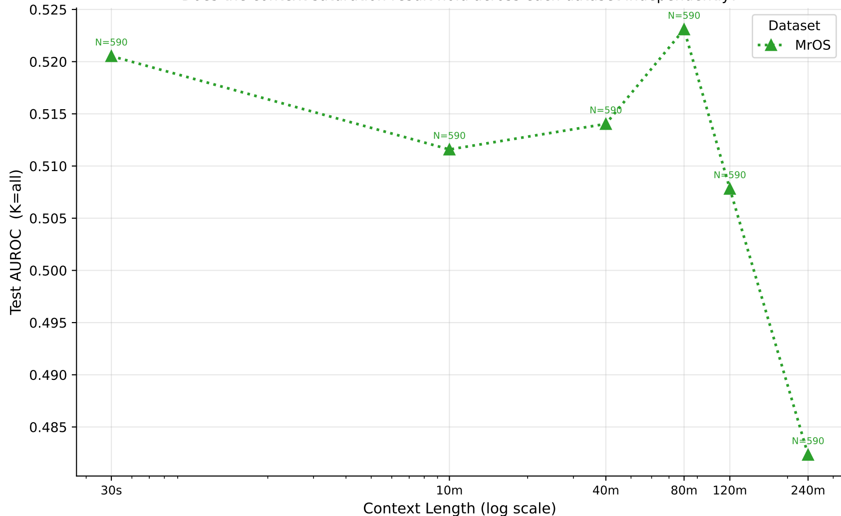
Cohort-Stratified Saturation — psqi_binary (LSTM) Does the context saturation result hold across each dataset independently?
