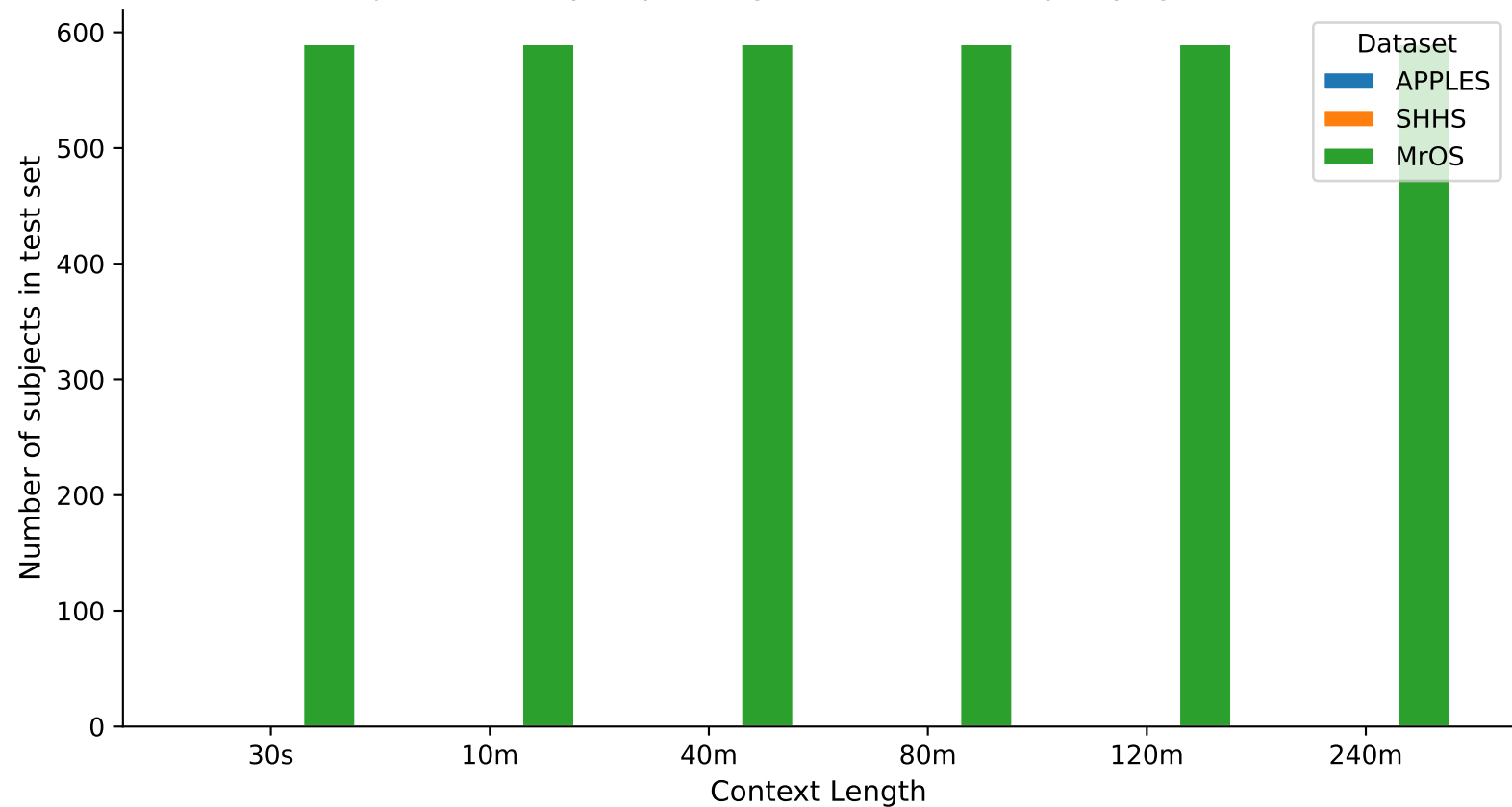
Test-Set Subject Count per Dataset — psqi_binary (LSTM) Subject count may drop at longer contexts (fewer qualifying windows)
