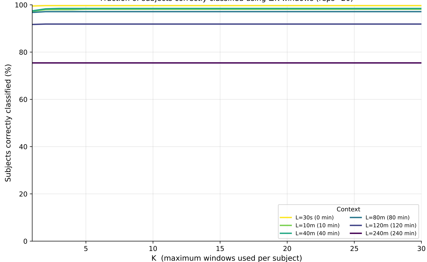
Coverage Curves — psqi_binary (LSTM) Fraction of subjects correctly classified using \leq K windows (reps=20)
