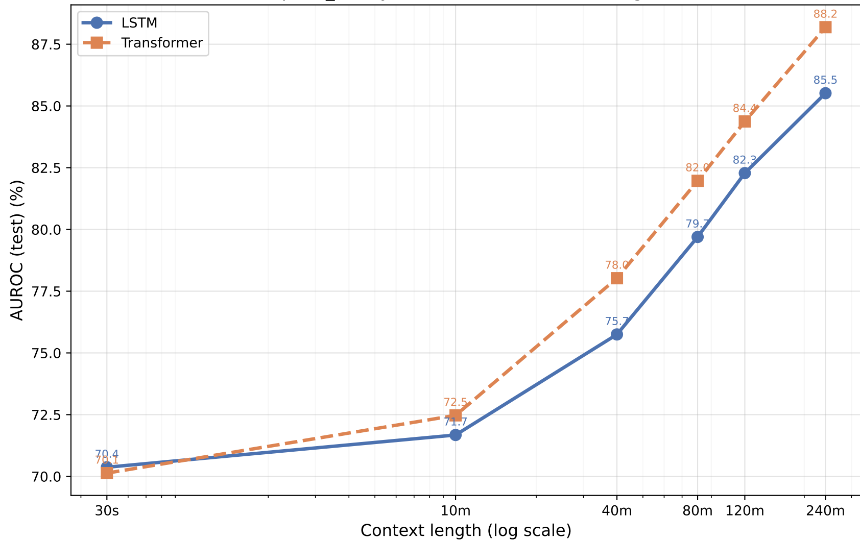
apnea_binary — AUROC vs Context Length
