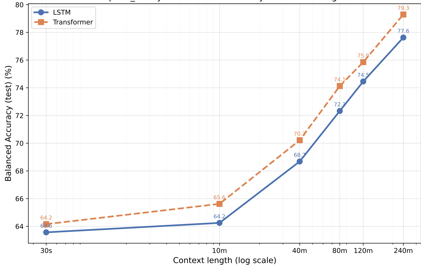
apnea_binary — Balanced Accuracy vs Context Length
