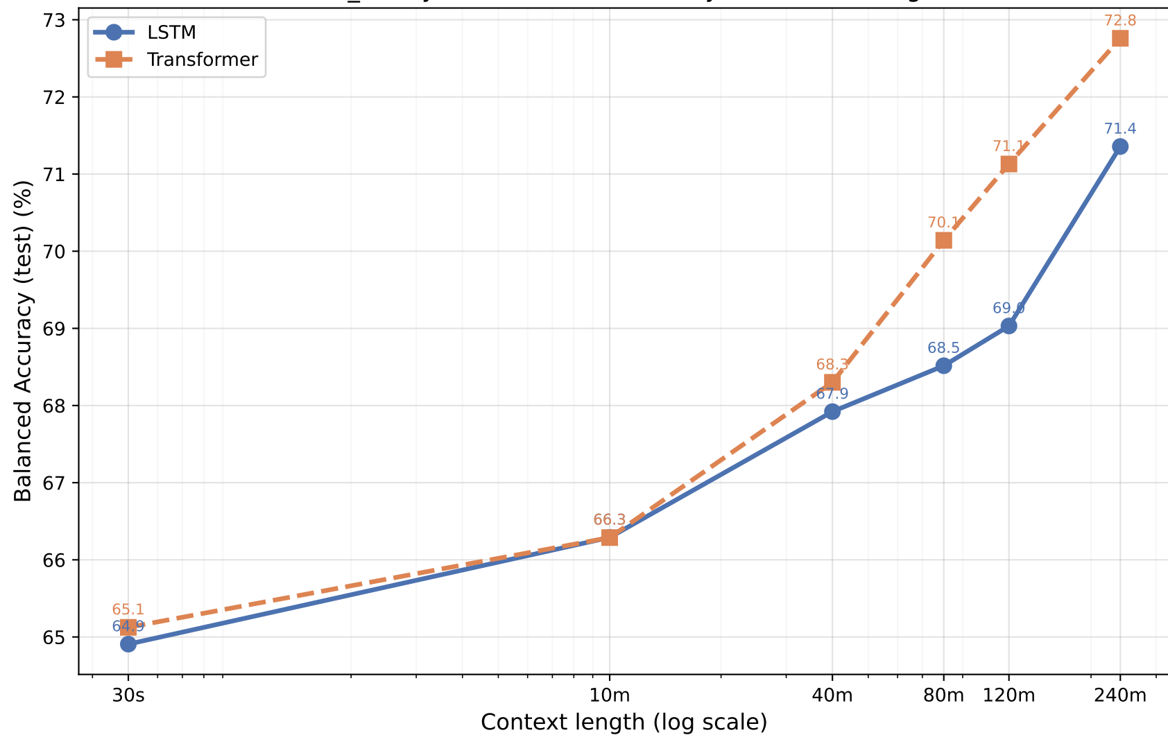
bmi_binary — Balanced Accuracy vs Context Length
