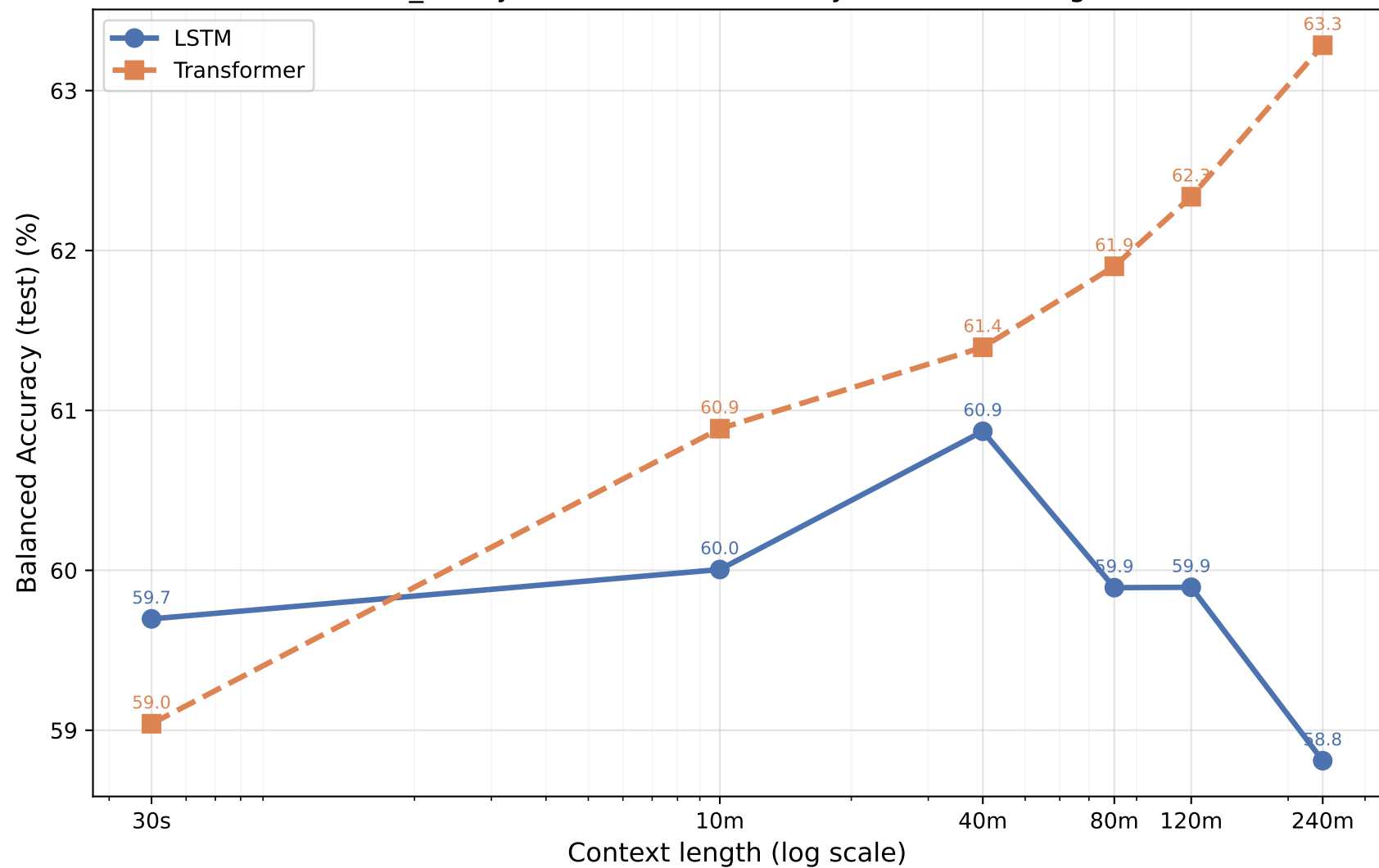
cvd_binary — Balanced Accuracy vs Context Length
