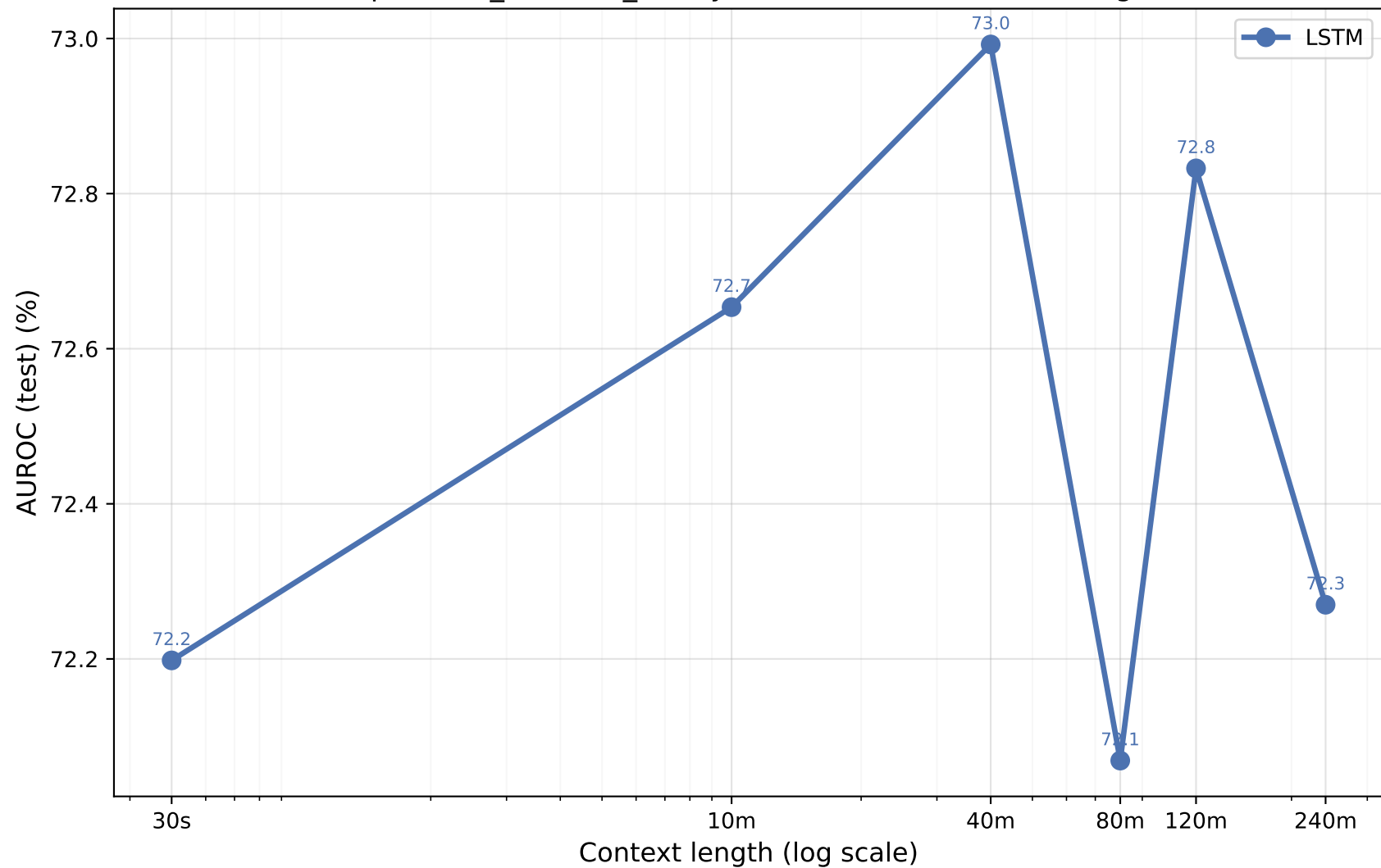
depression_extreme_binary — AUROC vs Context Length
