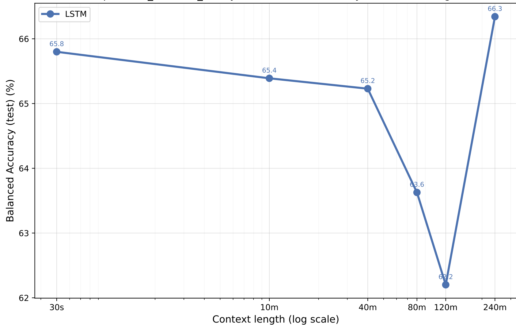
depression_extreme_binary — Balanced Accuracy vs Context Length
