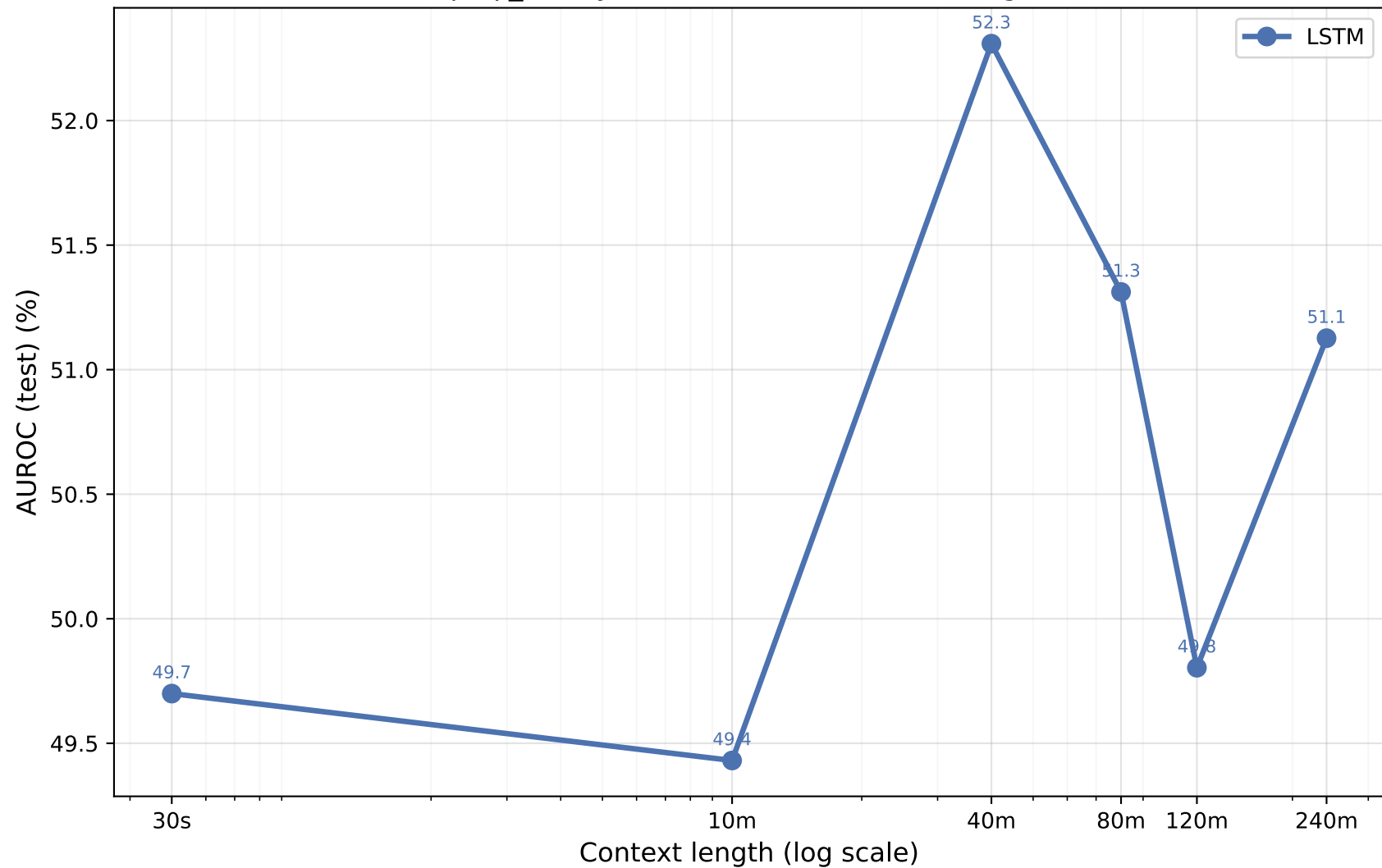
psqi_binary — AUROC vs Context Length
