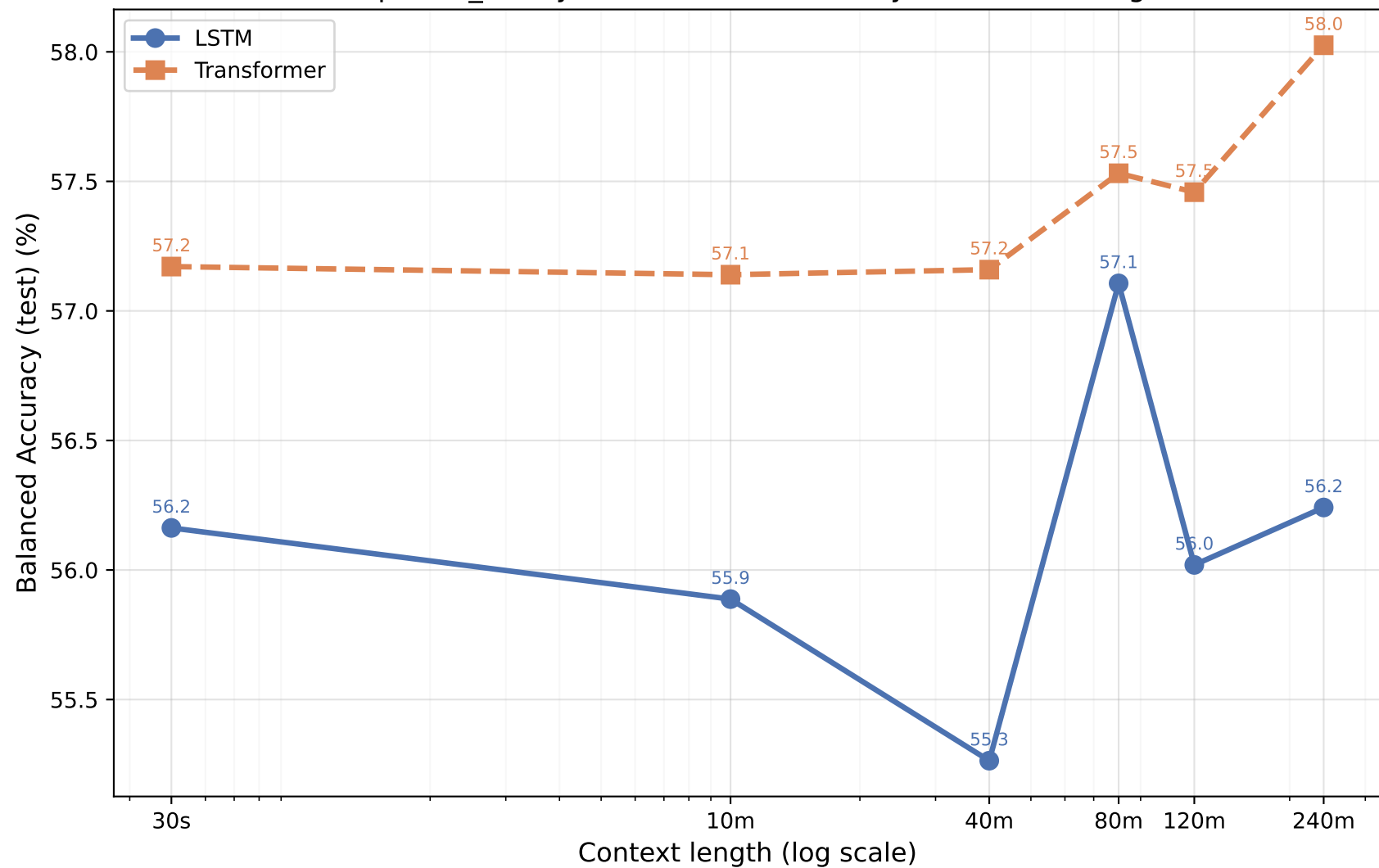
sleepiness_binary — Balanced Accuracy vs Context Length
