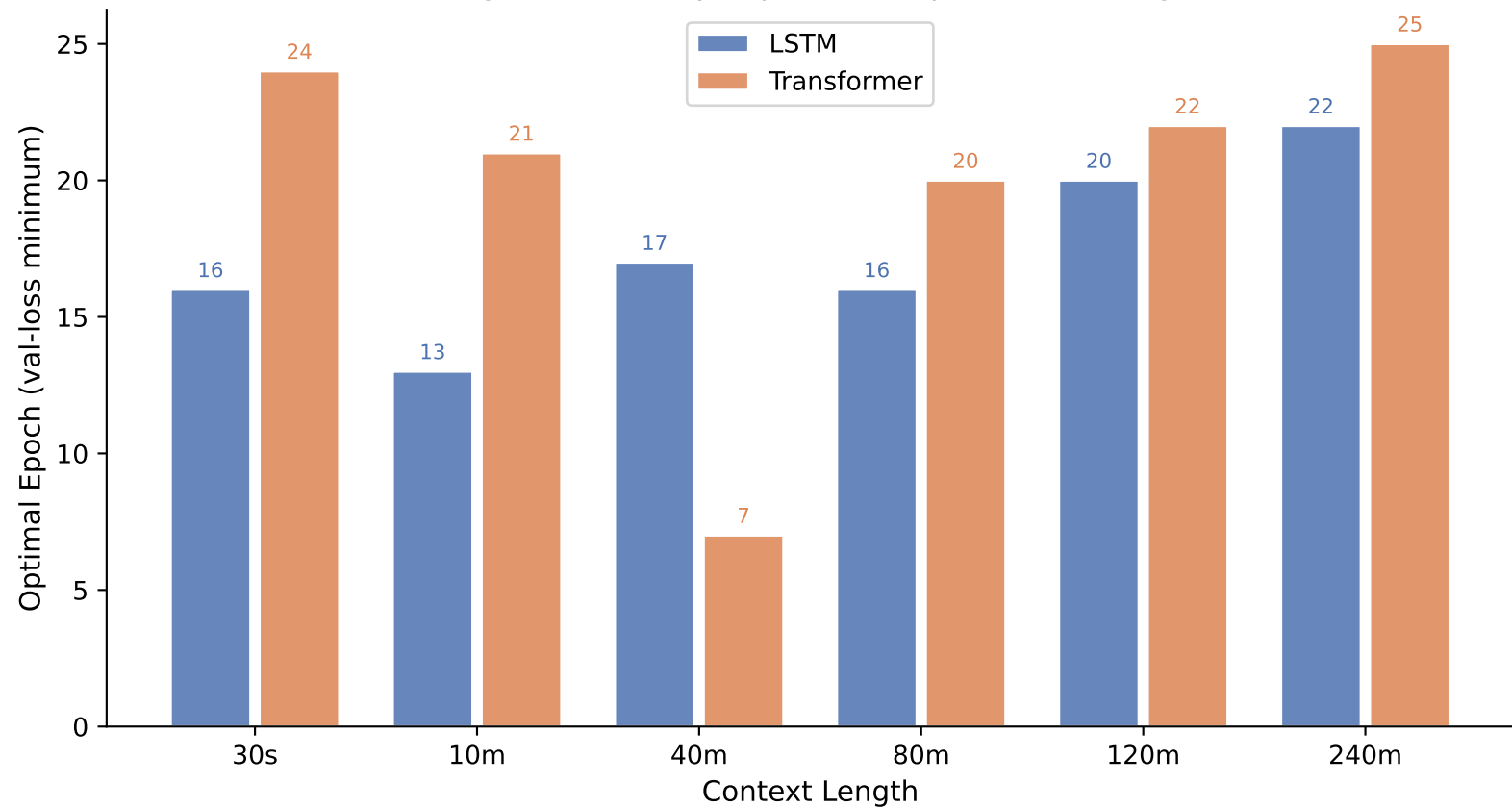
Optimal Epoch vs Context Length — age_class Longer context may require more epochs to converge
