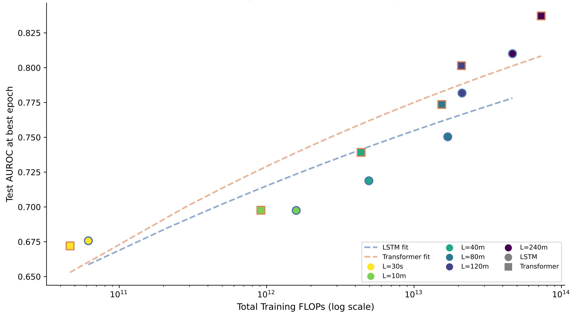
Compute Scaling Law — apnea_binary Color = context length · Marker = head · Dashed = power-law fit
