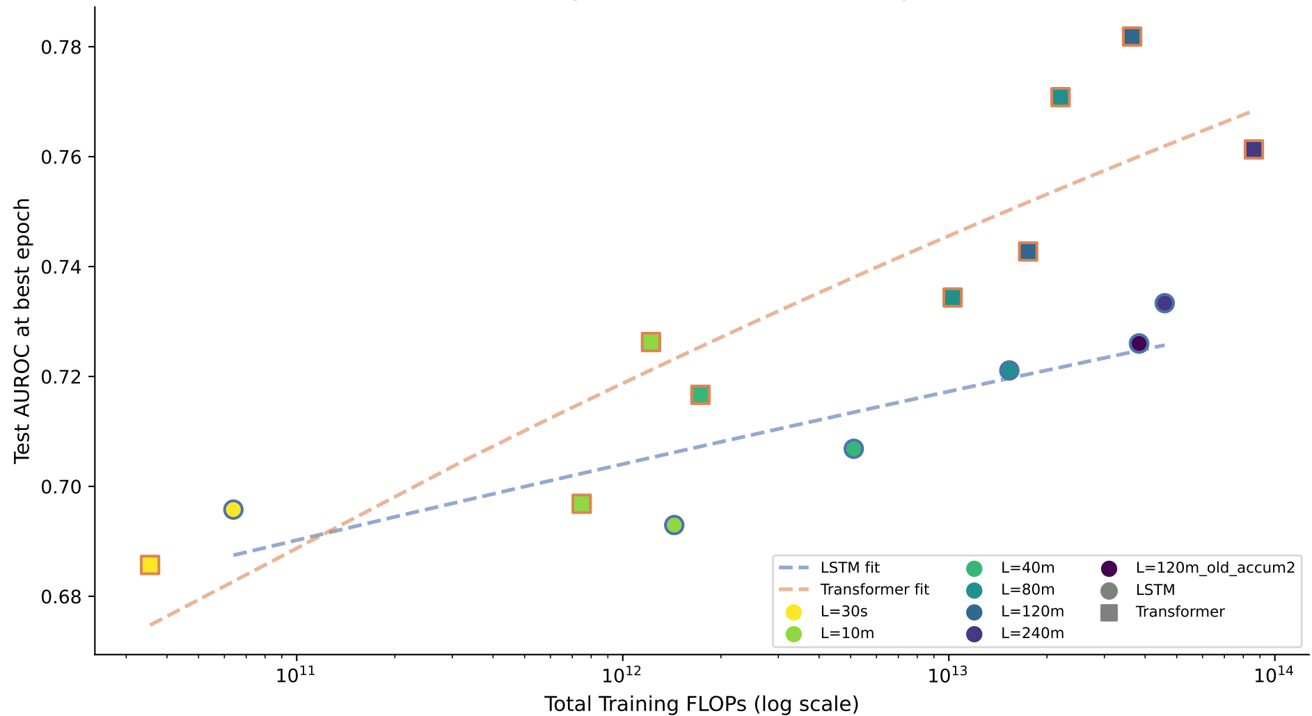
Compute Scaling Law — bmi_binary Color = context length · Marker = head · Dashed = power-law fit
