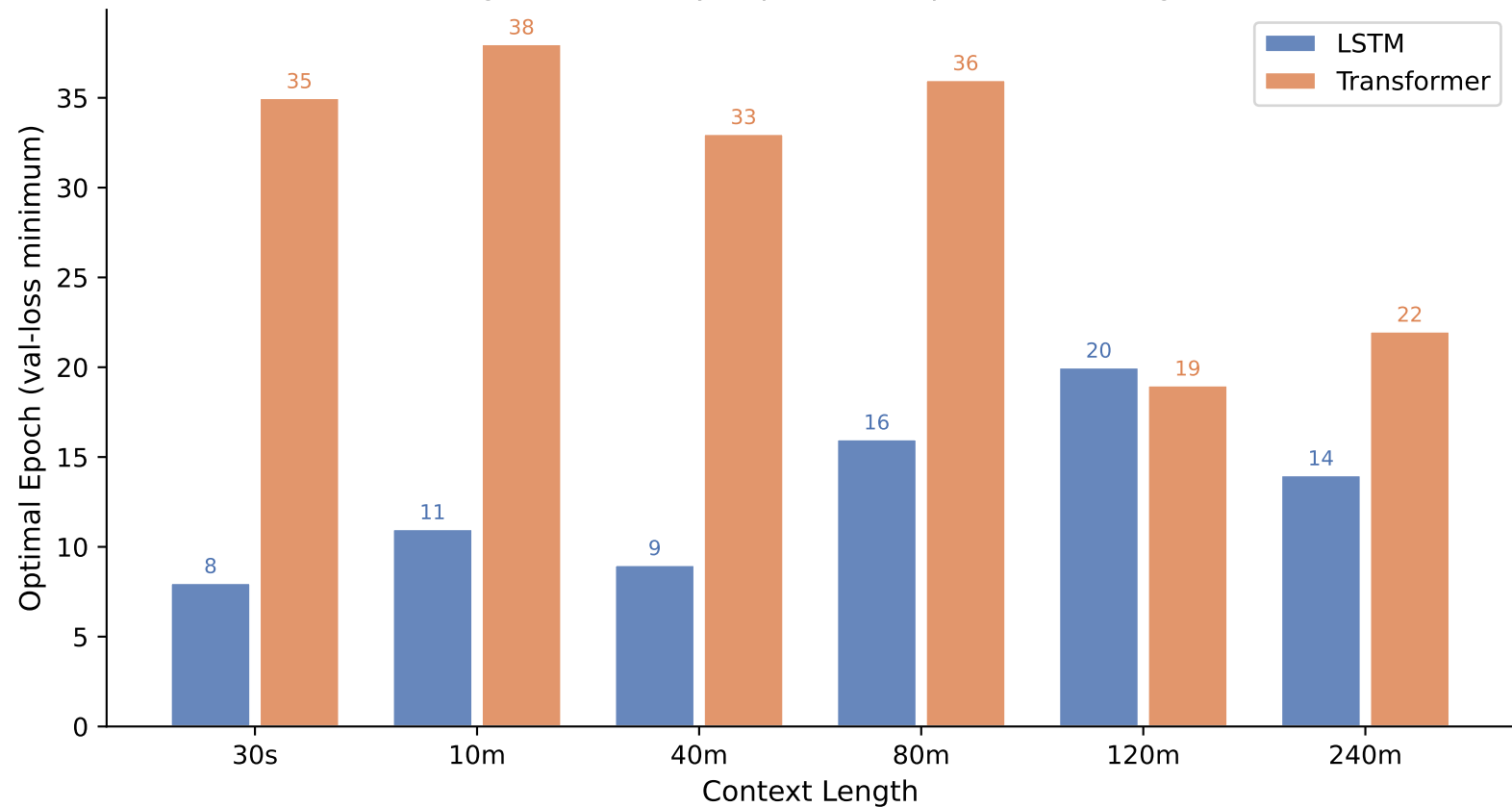
Optimal Epoch vs Context Length — sex_binary Longer context may require more epochs to converge
