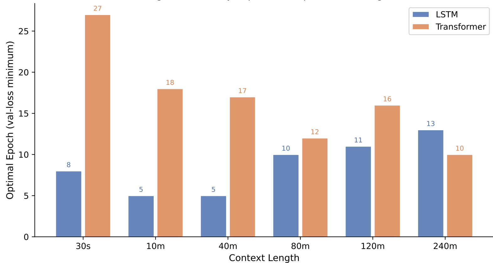
Optimal Epoch vs Context Length — sleep_efficiency_binary Longer context may require more epochs to converge
