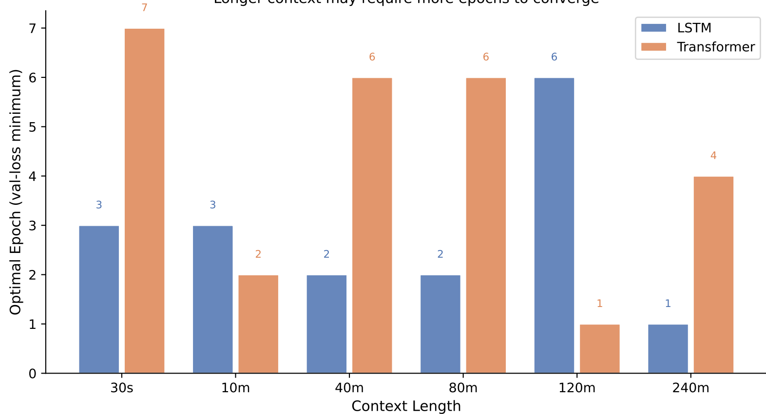
Optimal Epoch vs Context Length — sleepiness_binary Longer context may require more epochs to converge
