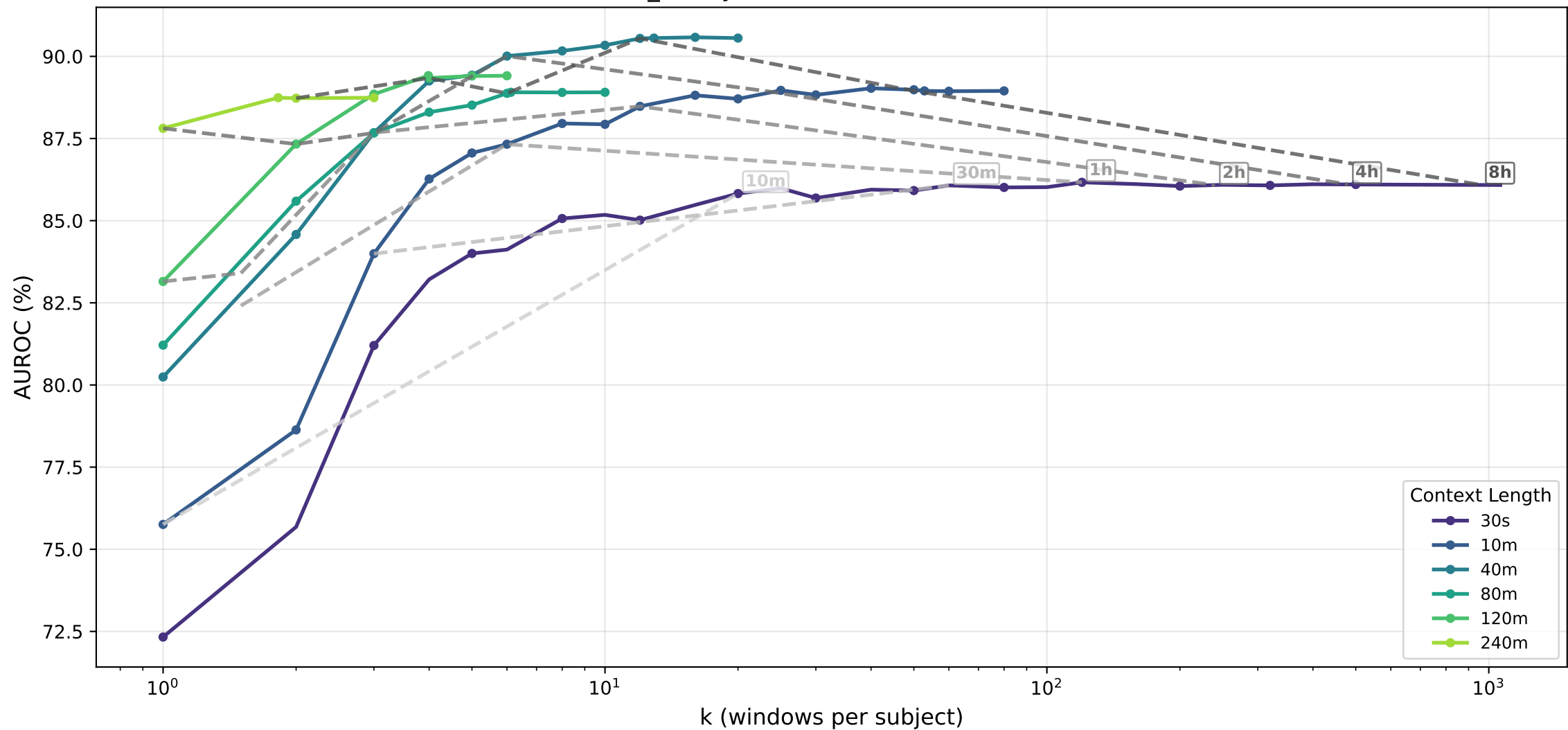
sex_binary · lstm — AUROC (%) vs k
