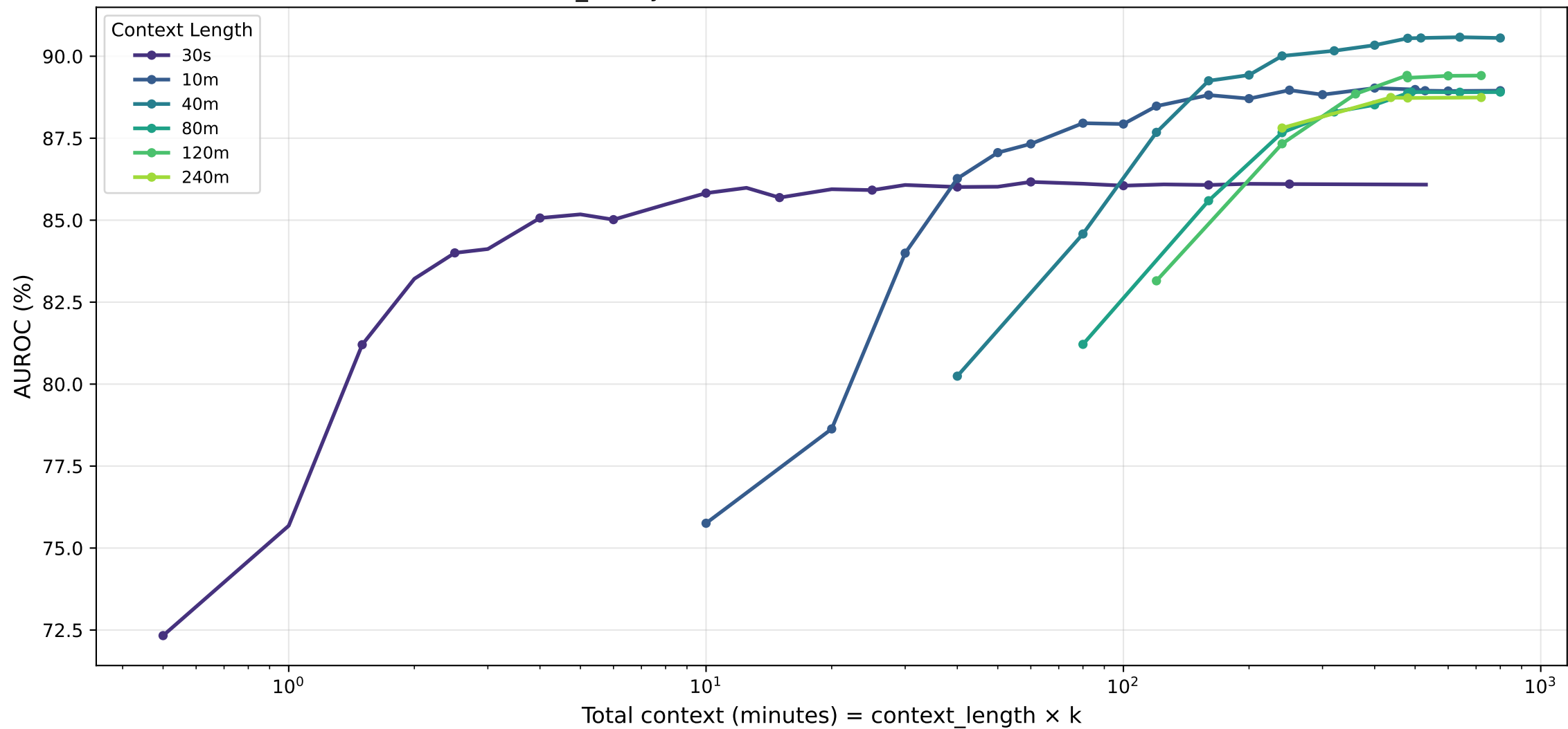
sex_binary · lstm — AUROC (%) vs Total Context
