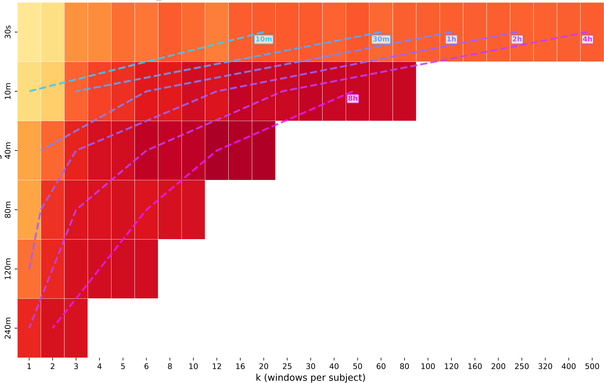
sex_binary · lstm — Iso-Compute Heatmap: Balanced Accuracy (%)
