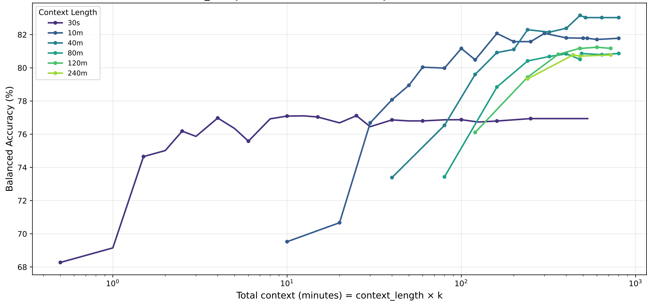
sex_binary · lstm — Balanced Accuracy (%) vs Total Context
