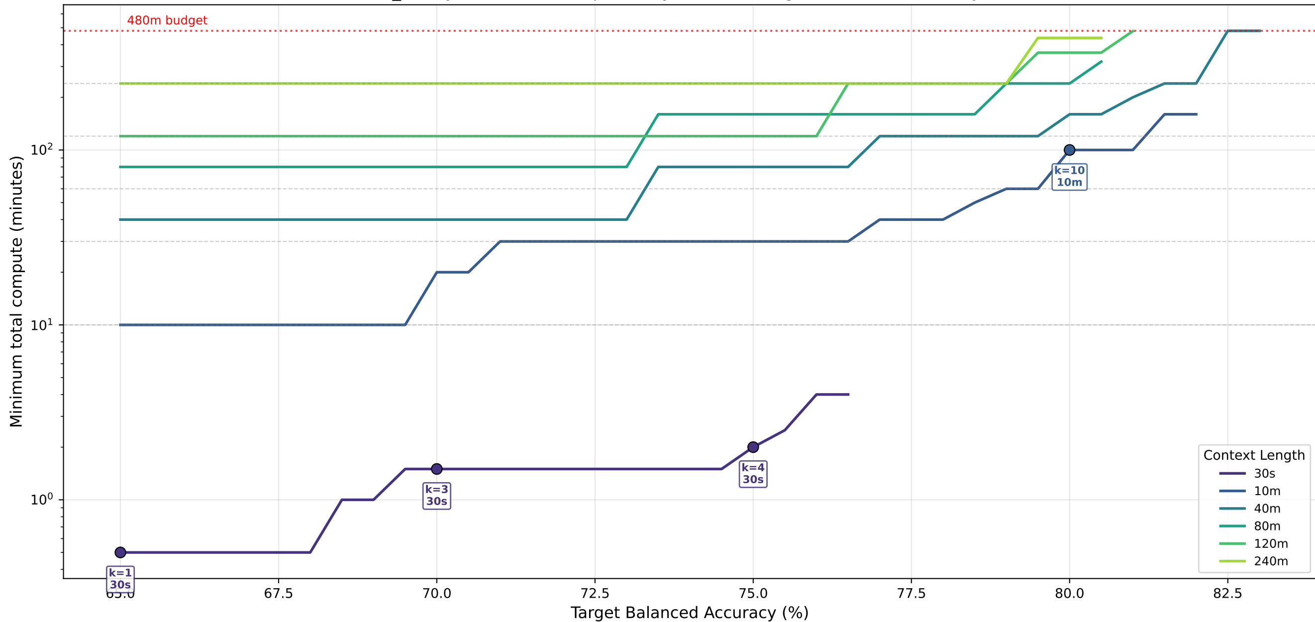
sex_binary · lstm — Cheapest Way to Reach Target Balanced Accuracy (%)
