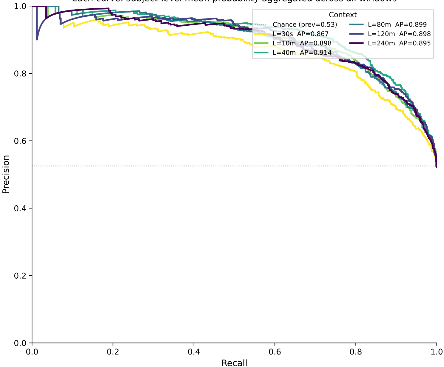
Precision-Recall Curves — sex_binary (LSTM) K=all Each curve: subject-level mean probability aggregated across all windows
