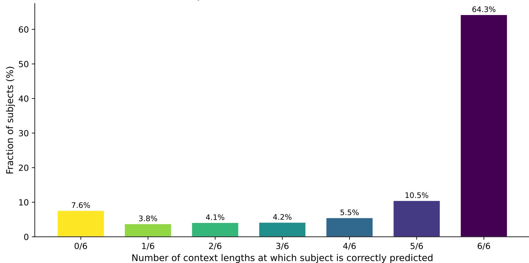
Hard-Subject Analysis — sex_binary (LSTM) N = 1430 subjects · 0/6 = never correct (irreducible hard cases)
