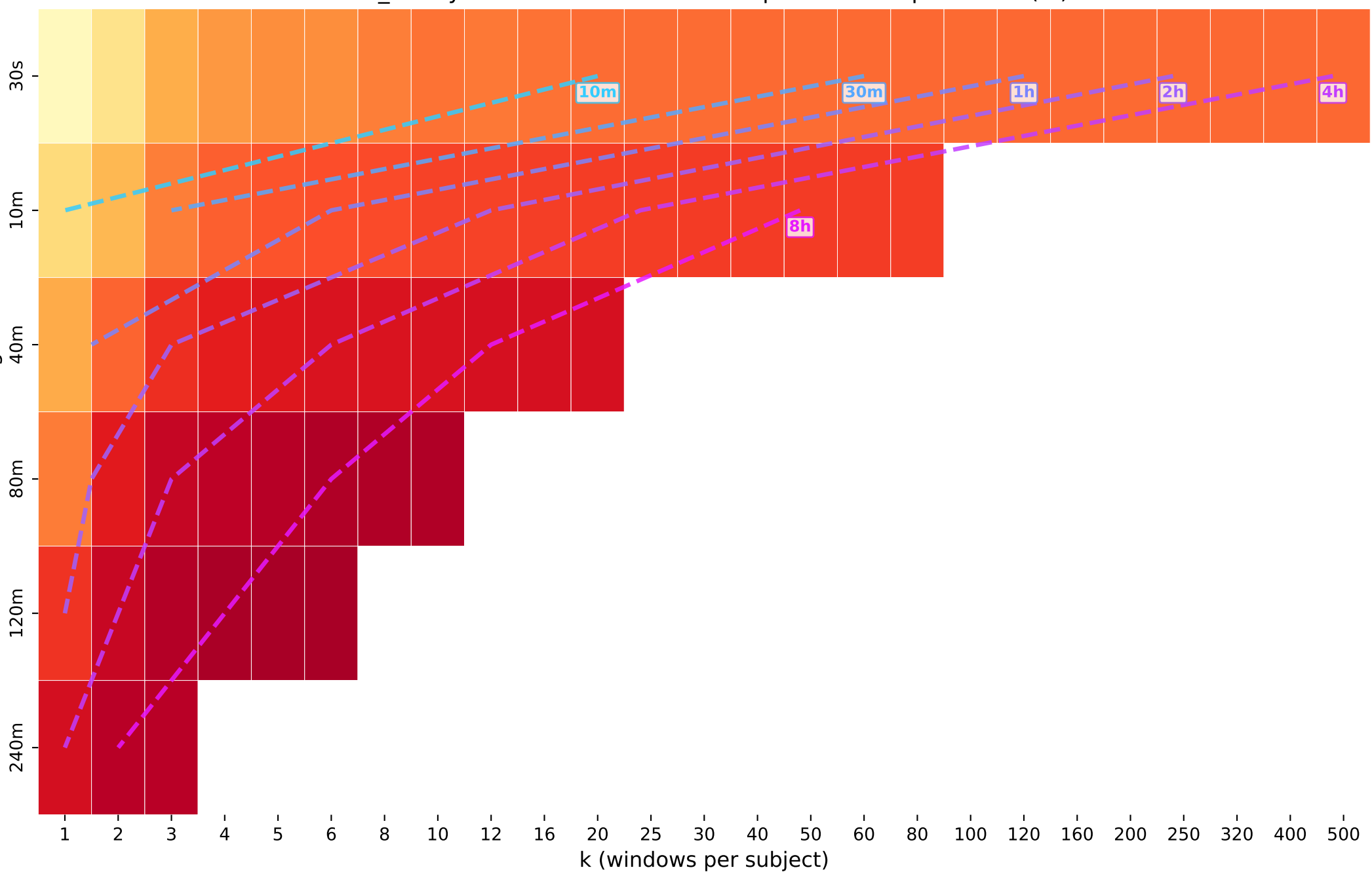
sex_binary · transformer — Iso-Compute Heatmap: AUROC (%)
