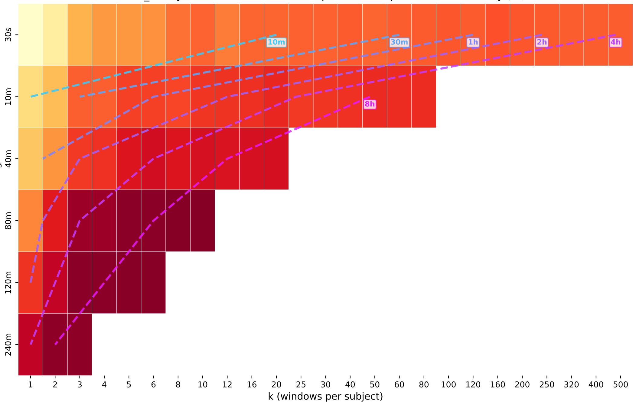
sex_binary · transformer — Iso-Compute Heatmap: Balanced Accuracy (%)
