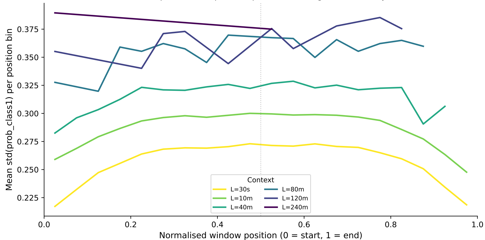
Prediction Variance vs Night Position — sex_binary (TRANSFORMER) Lower variance = position-independent predictions (longer context may flatten this)
