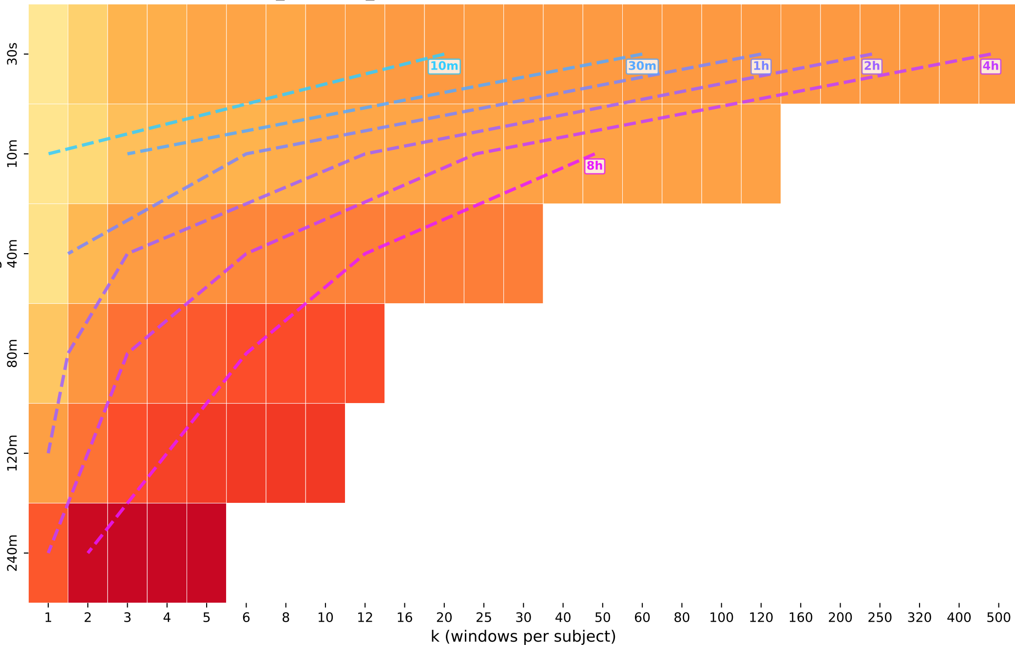
sleep_efficiency_binary · lstm — Iso-Compute Heatmap: AUROC (%)
