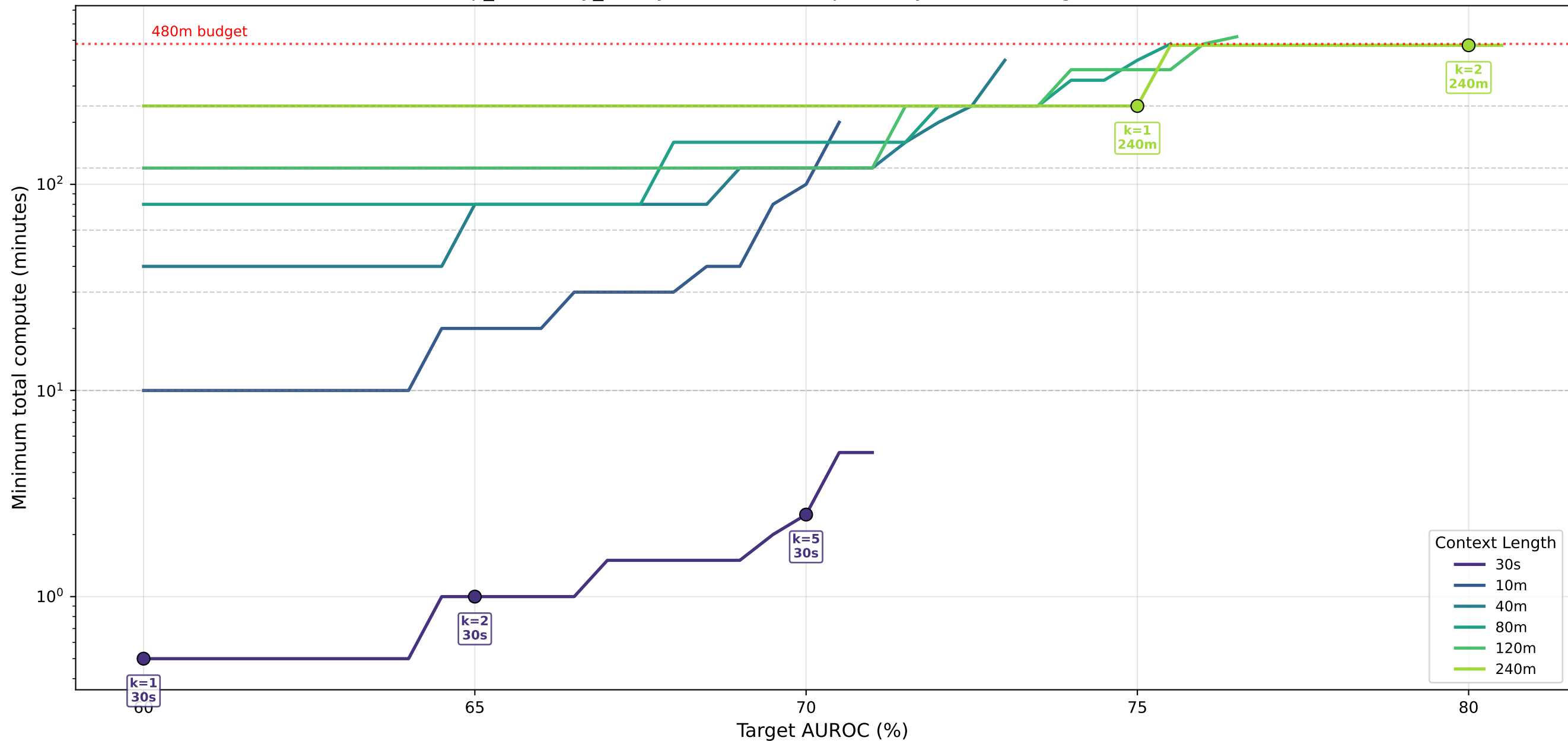
sleep_efficiency_binary · lstm — Cheapest Way to Reach Target AUROC (%)
