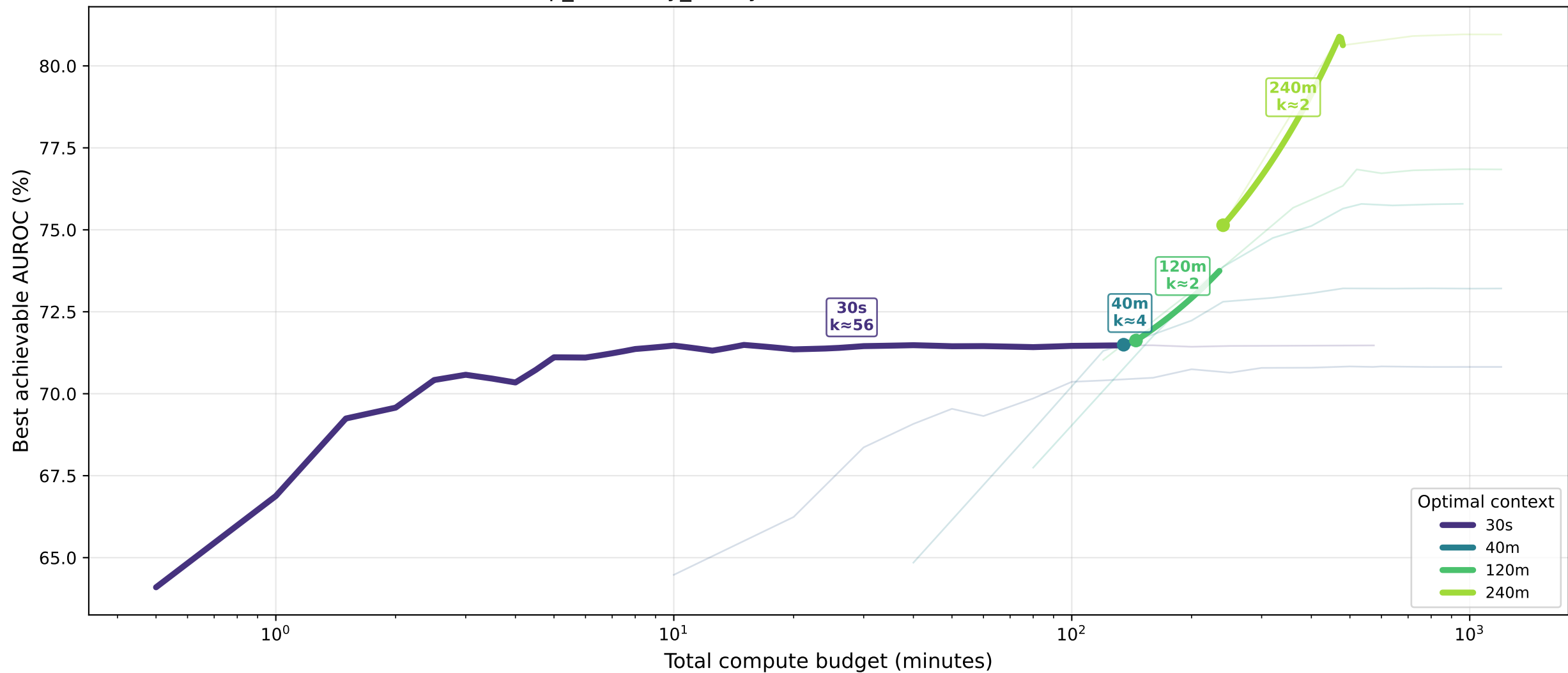
sleep_efficiency_binary · lstm — Pareto Front: AUROC (%)
