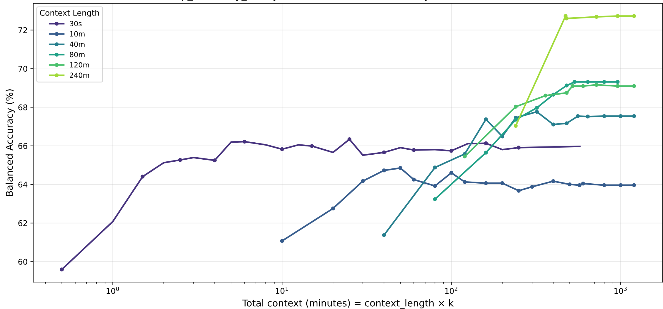
sleep_efficiency_binary · lstm — Balanced Accuracy (%) vs Total Context
