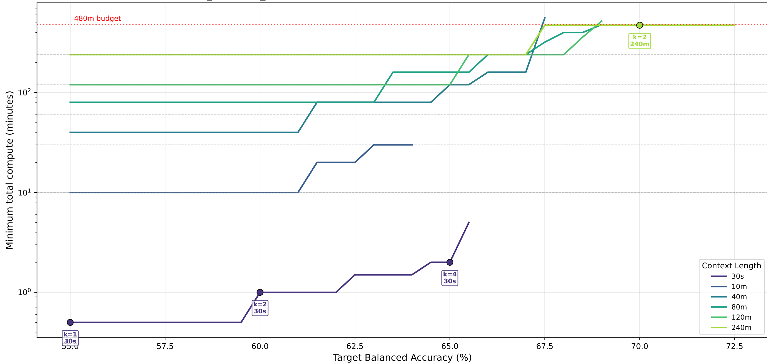
sleep_efficiency_binary · lstm — Cheapest Way to Reach Target Balanced Accuracy (%)
