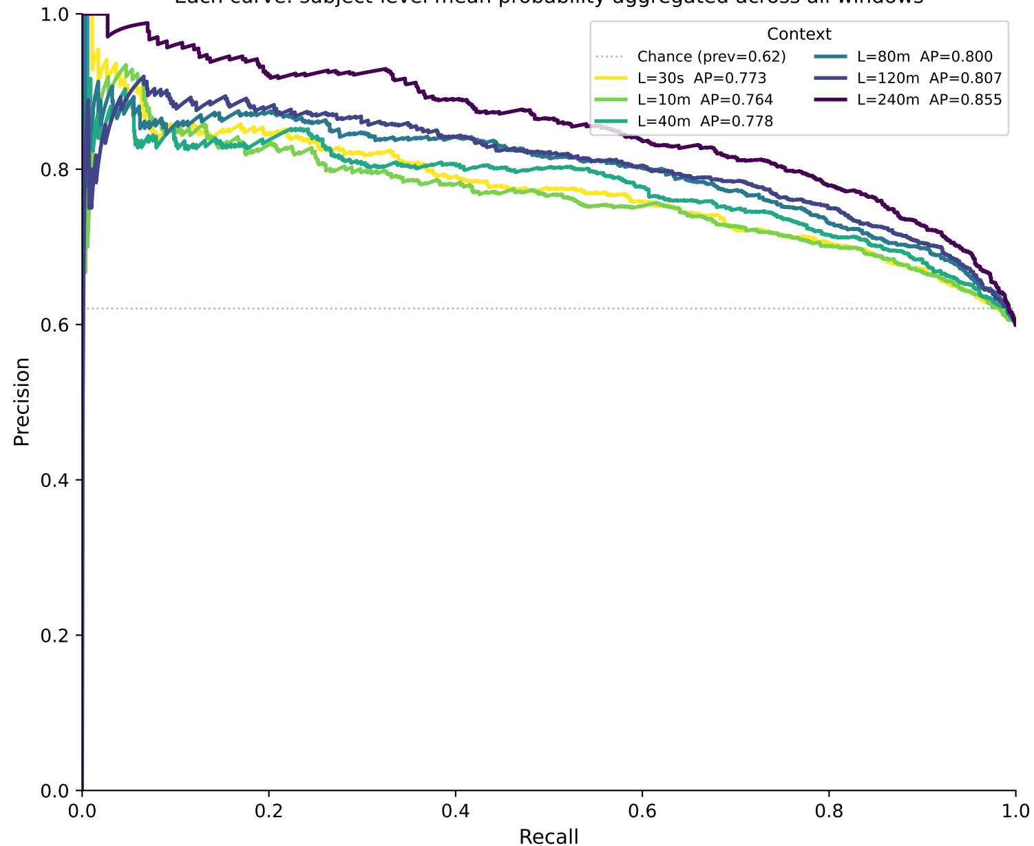
Precision-Recall Curves — sleep_efficiency_binary (LSTM) K=all Each curve: subject-level mean probability aggregated across all windows
