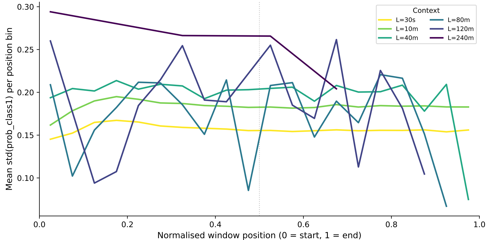
Prediction Variance vs Night Position — sleep_efficiency_binary (LSTM) Lower variance = position-independent predictions (longer context may flatten this)
