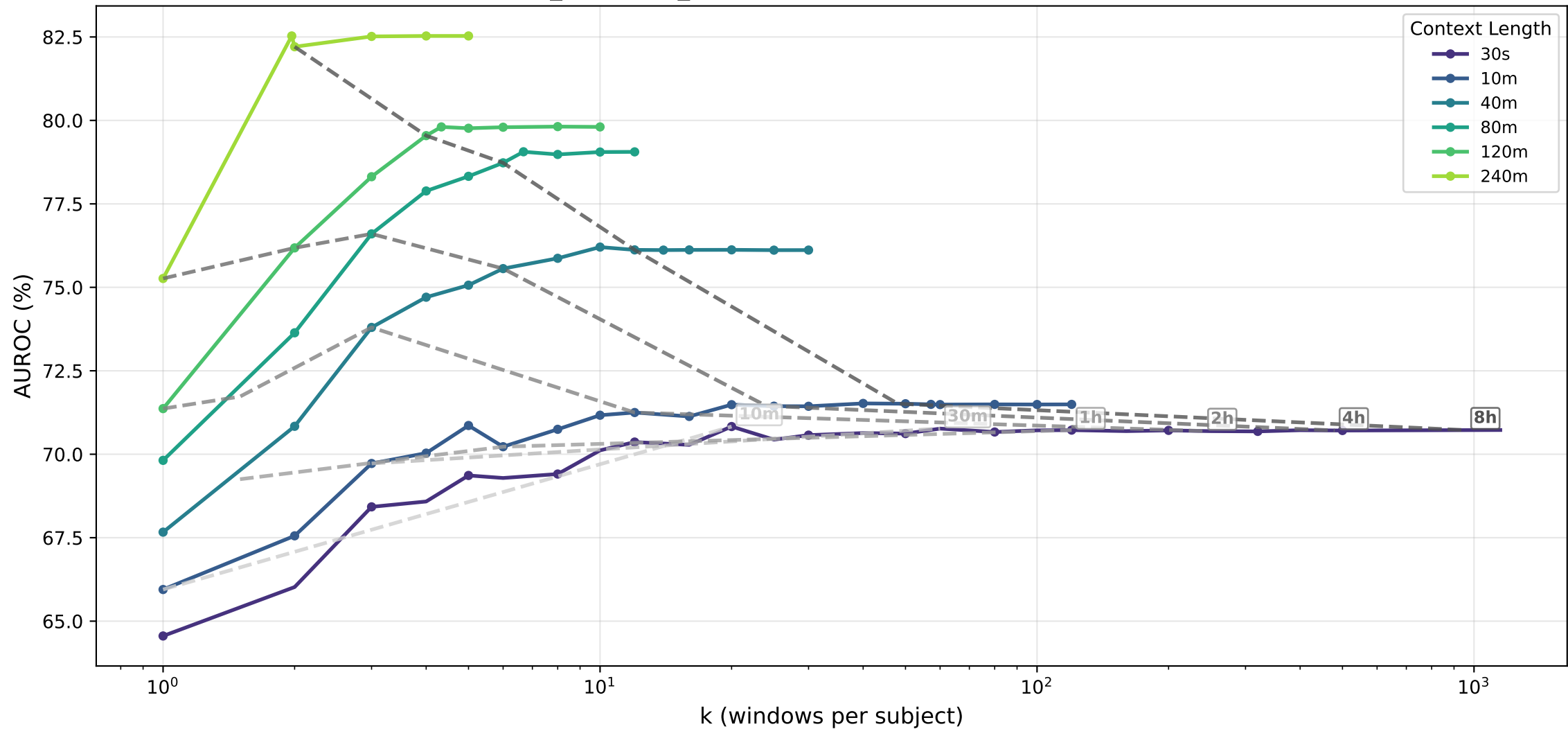
sleep_efficiency_binary · transformer — AUROC (%) vs k
