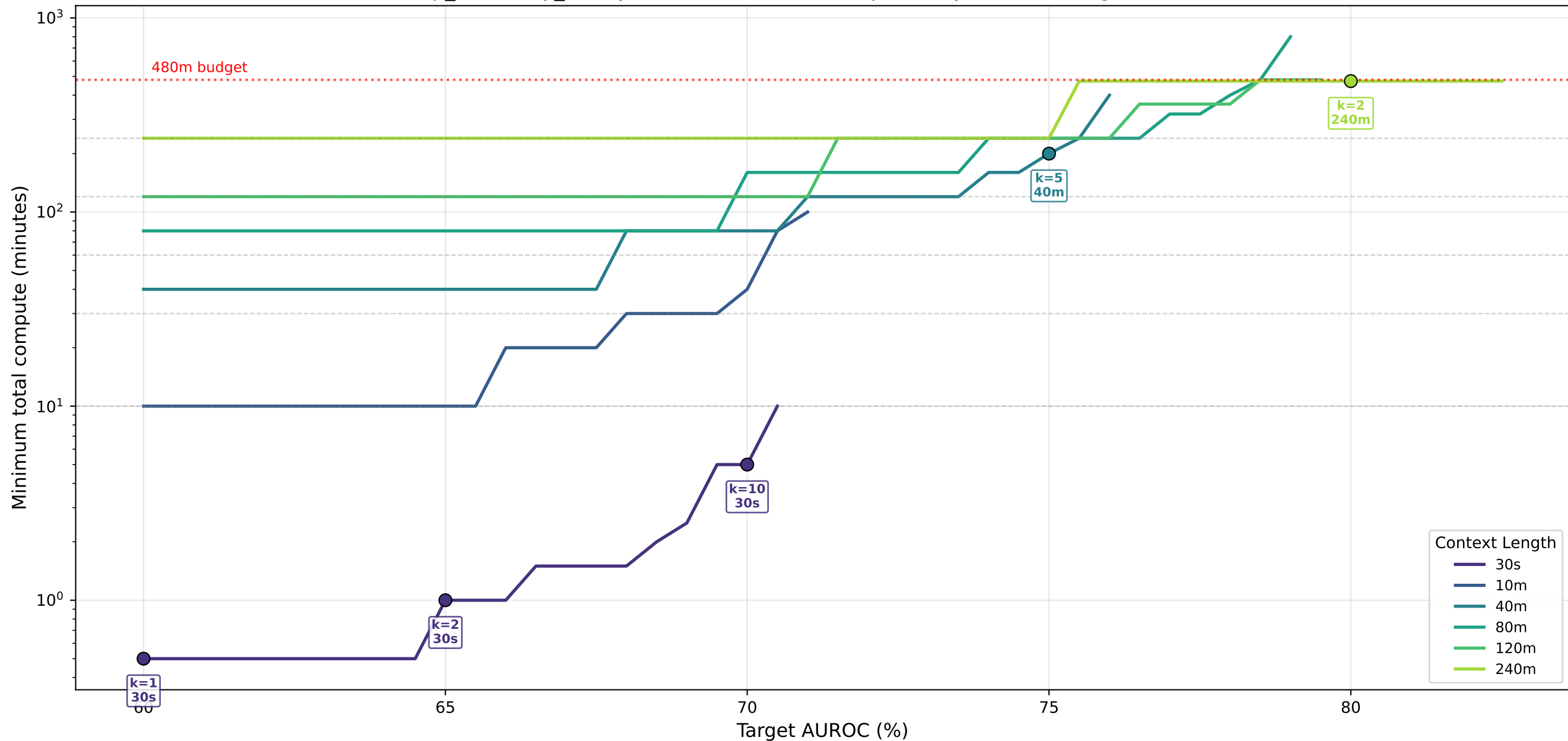
sleep_efficiency_binary · transformer — Cheapest Way to Reach Target AUROC (%)
