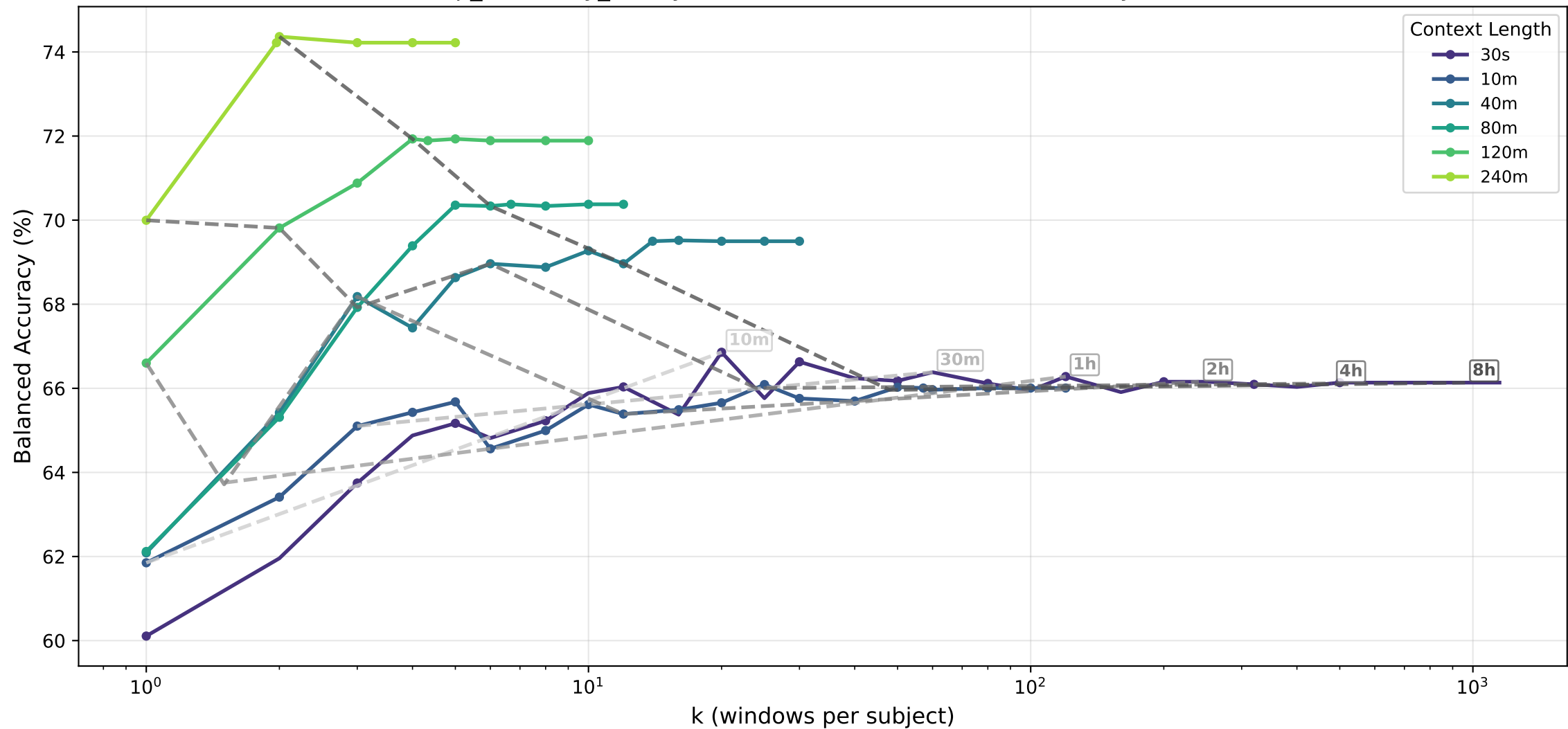
sleep_efficiency_binary · transformer — Balanced Accuracy (%) vs k
