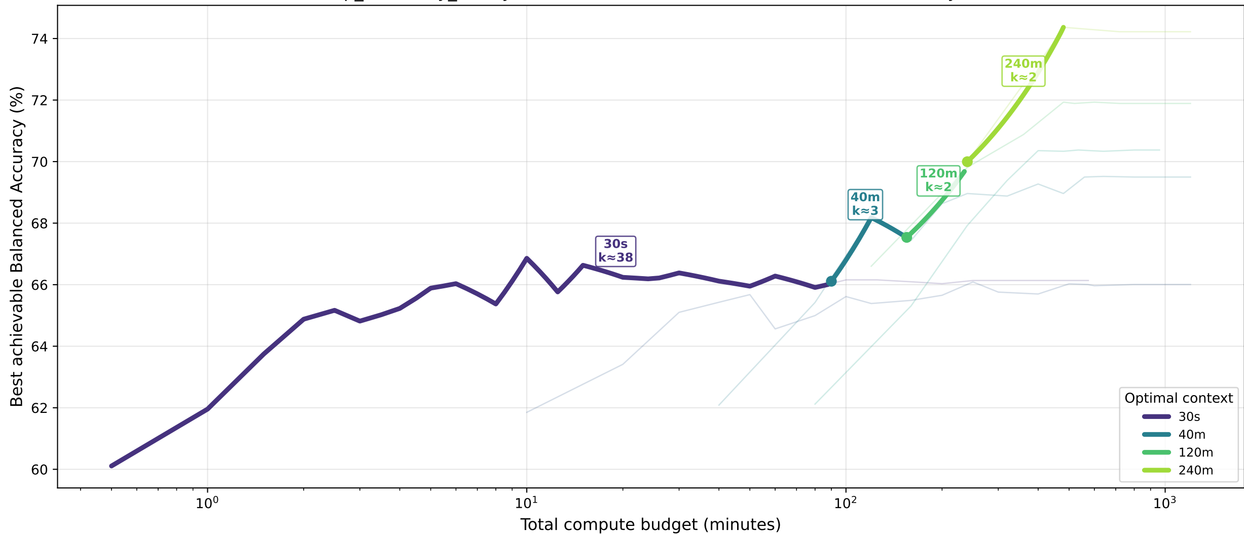
sleep_efficiency_binary · transformer — Pareto Front: Balanced Accuracy (%)
