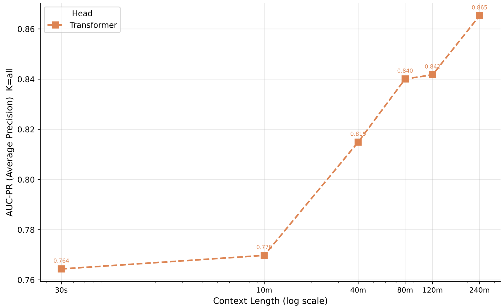
AUC-PR vs Context Length — sleep_efficiency_binary Does precision-recall performance saturate like AUROC?
