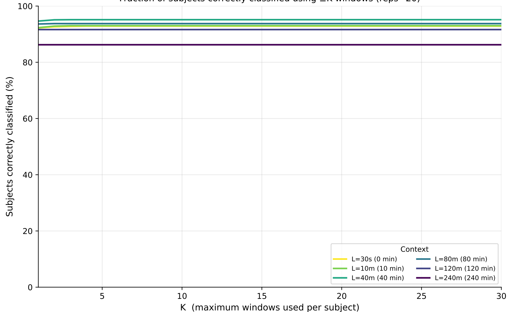
Coverage Curves — sleep_efficiency_binary (TRANSFORMER) Fraction of subjects correctly classified using \leq K windows (reps=20)
