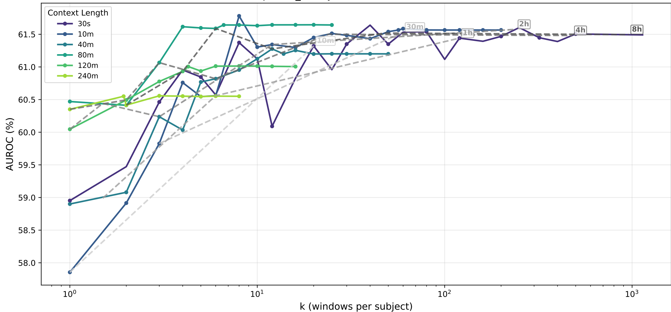
sleepiness_binary · lstm — AUROC (%) vs k
