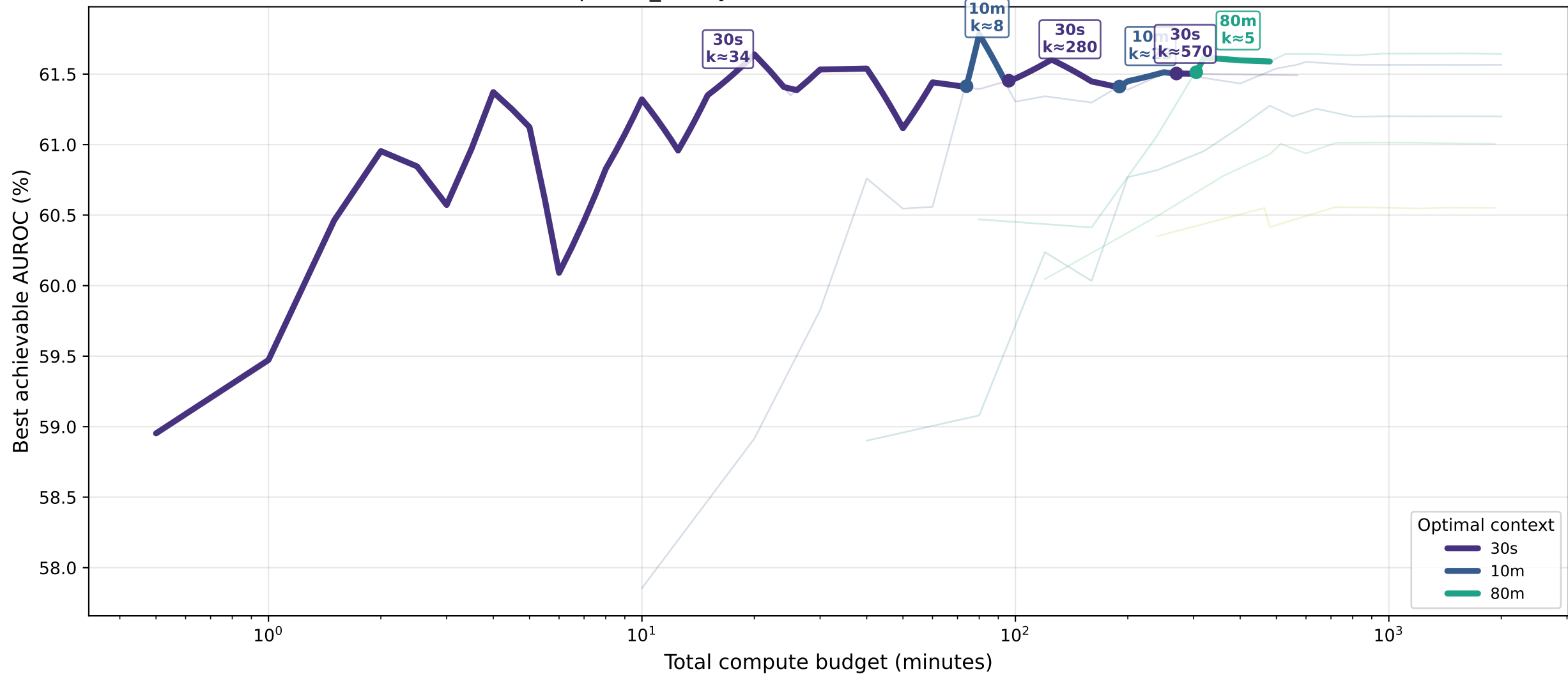
sleepiness_binary · lstm — Pareto Front: AUROC (%)
