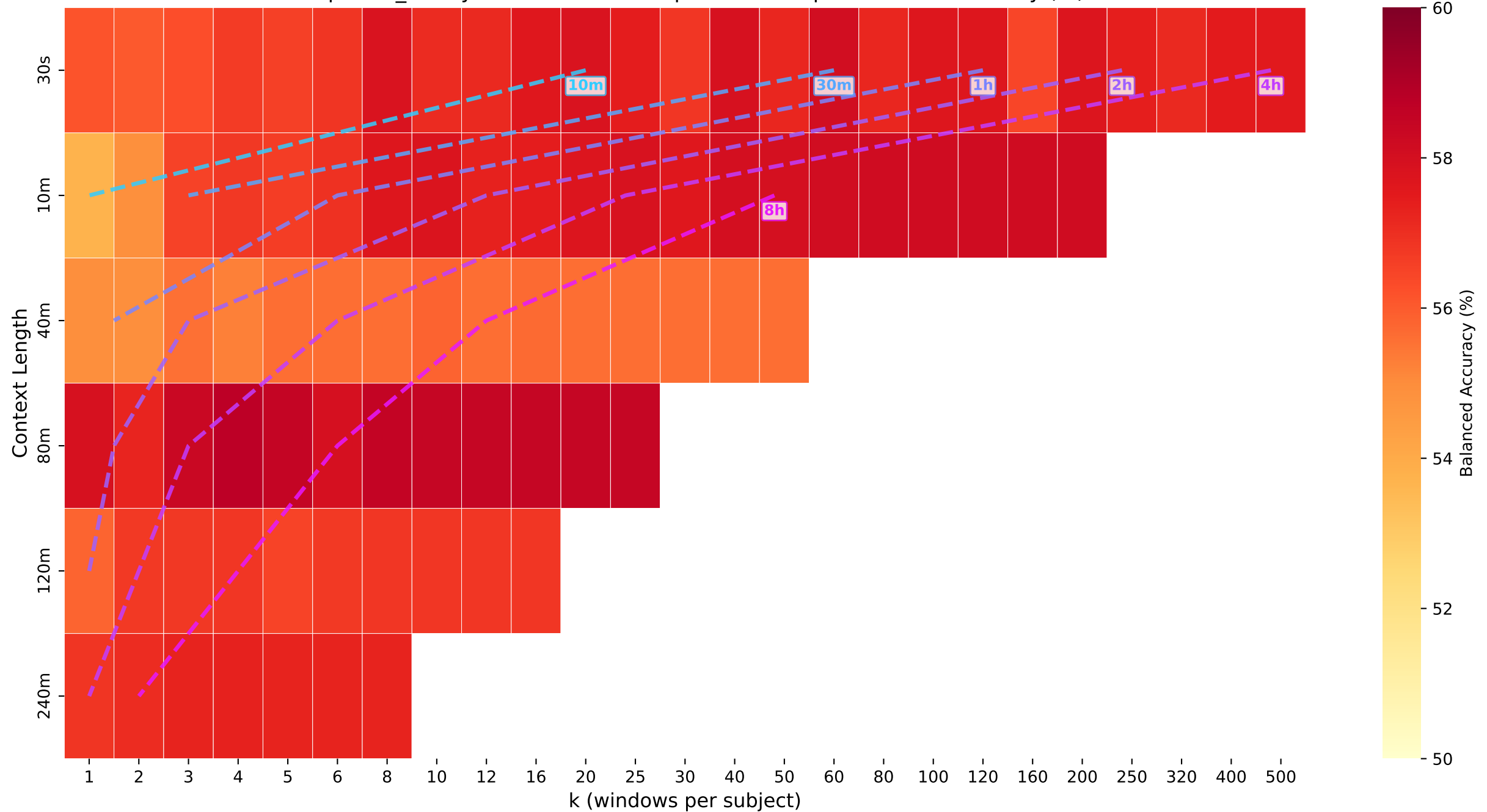
sleepiness_binary · lstm — Iso-Compute Heatmap: Balanced Accuracy (%)
