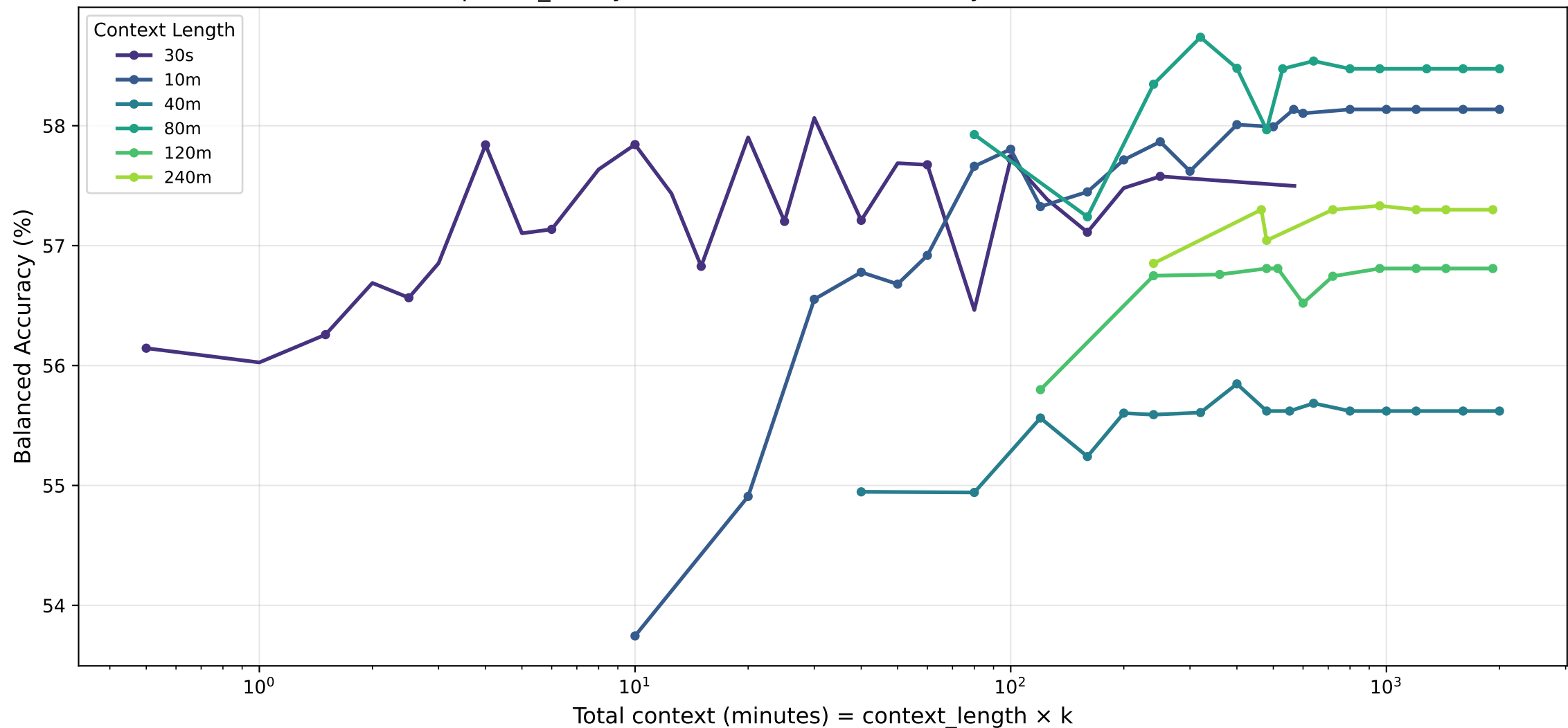
sleepiness_binary · Istml — Balanced Accuracy (%) vs Total Context
