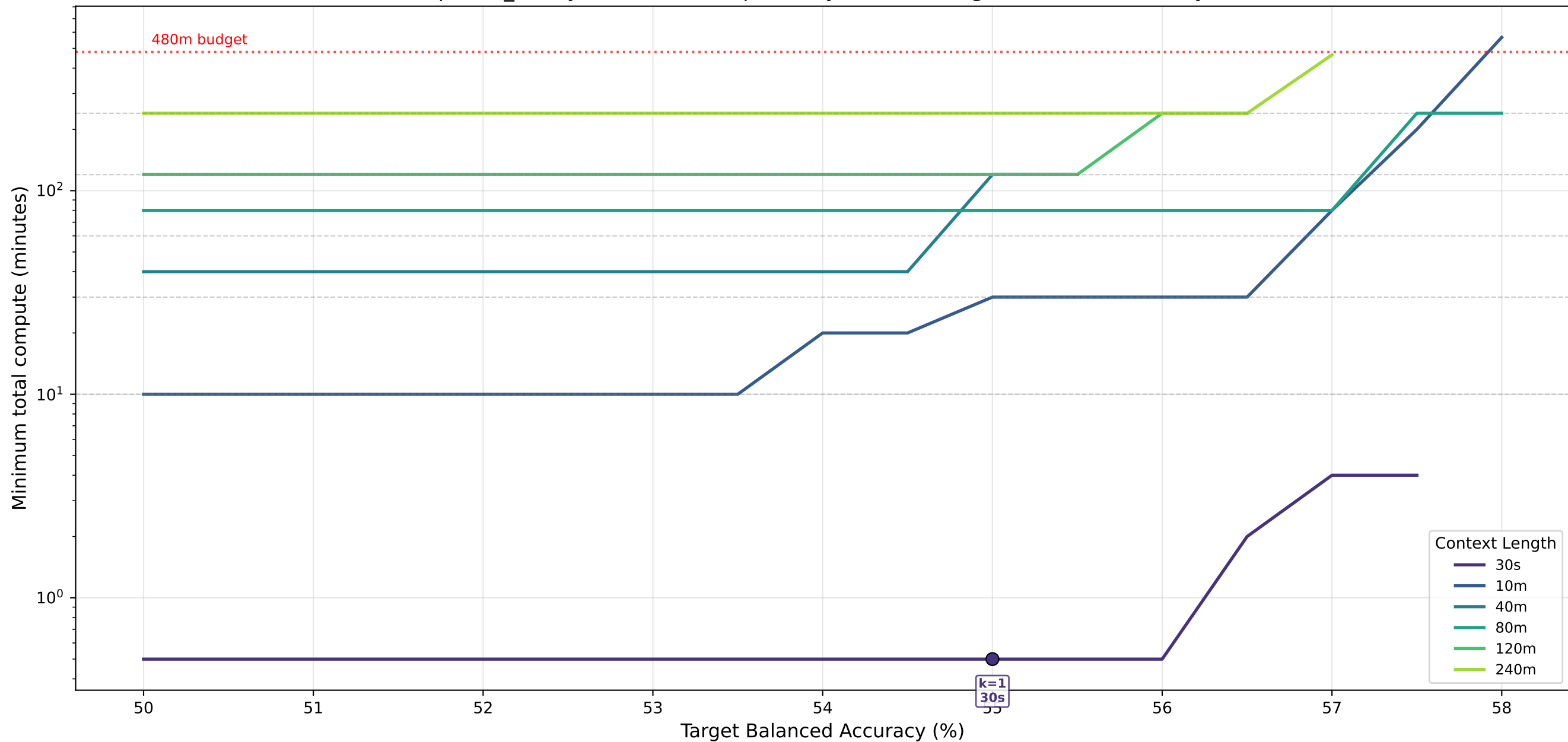
sleepiness_binary · lstm — Cheapest Way to Reach Target Balanced Accuracy (%)
